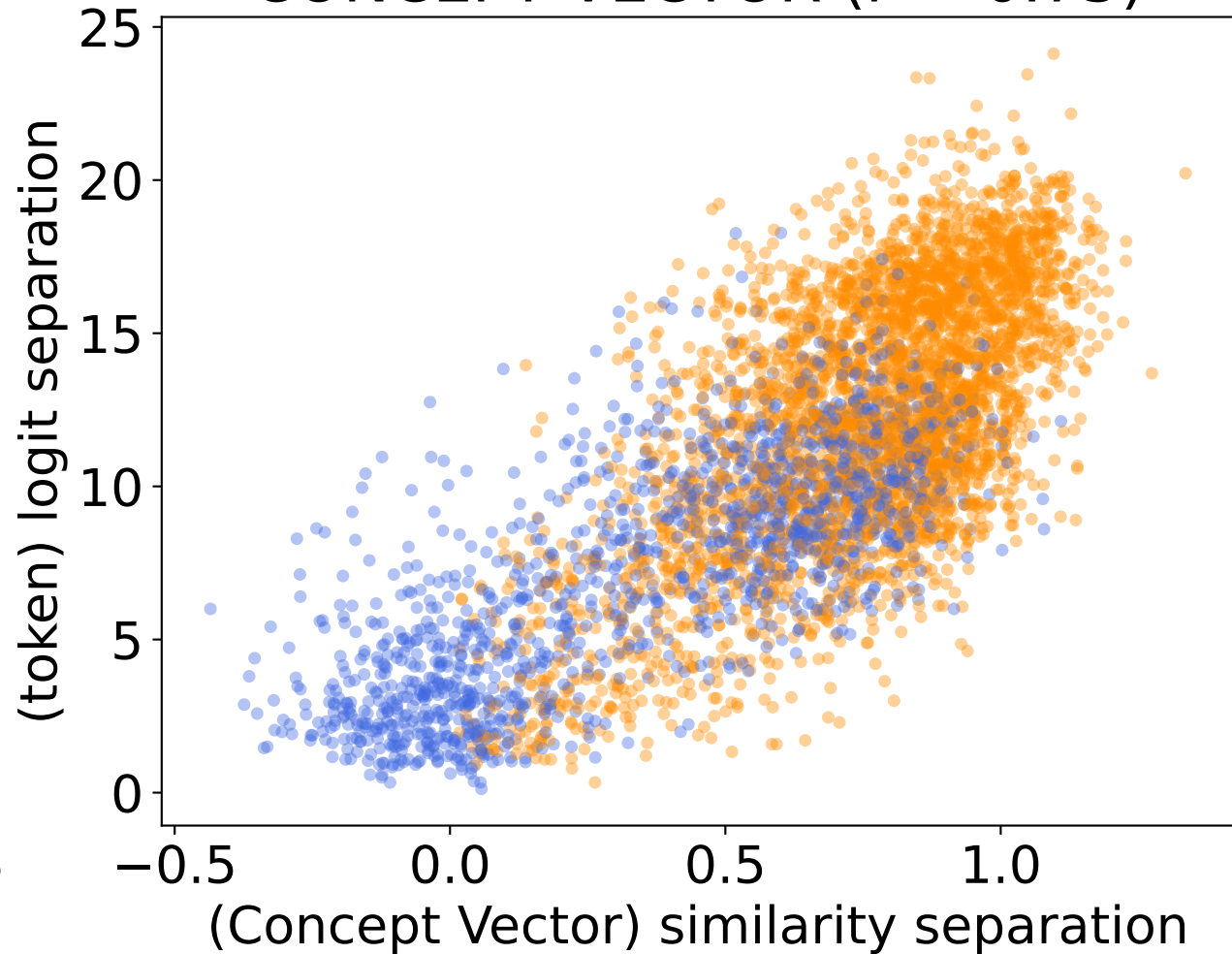
CONCEPT VECTOR ( r = 0.75 )
