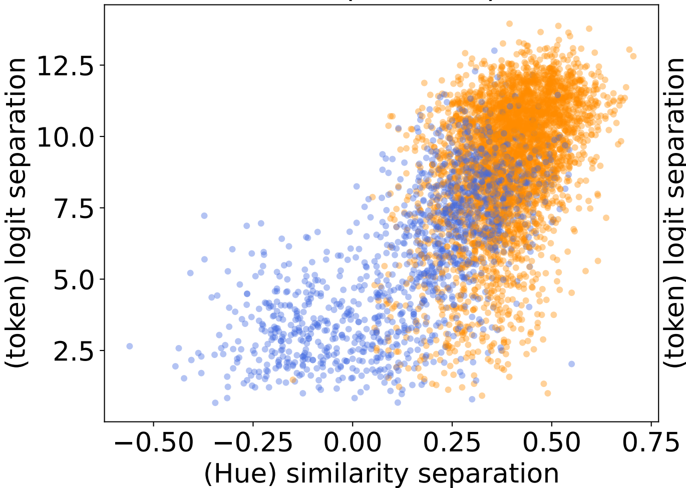
HUE ( r = 0.67 )
