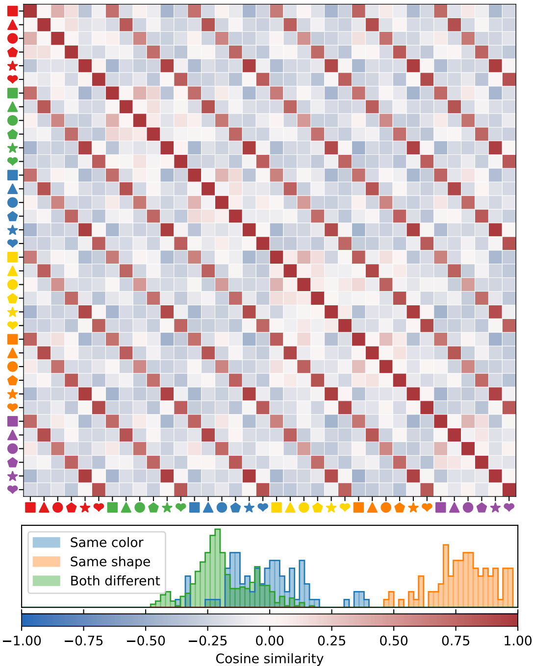
Gemma 3 12B - Centroid-Based Concept Vectors
