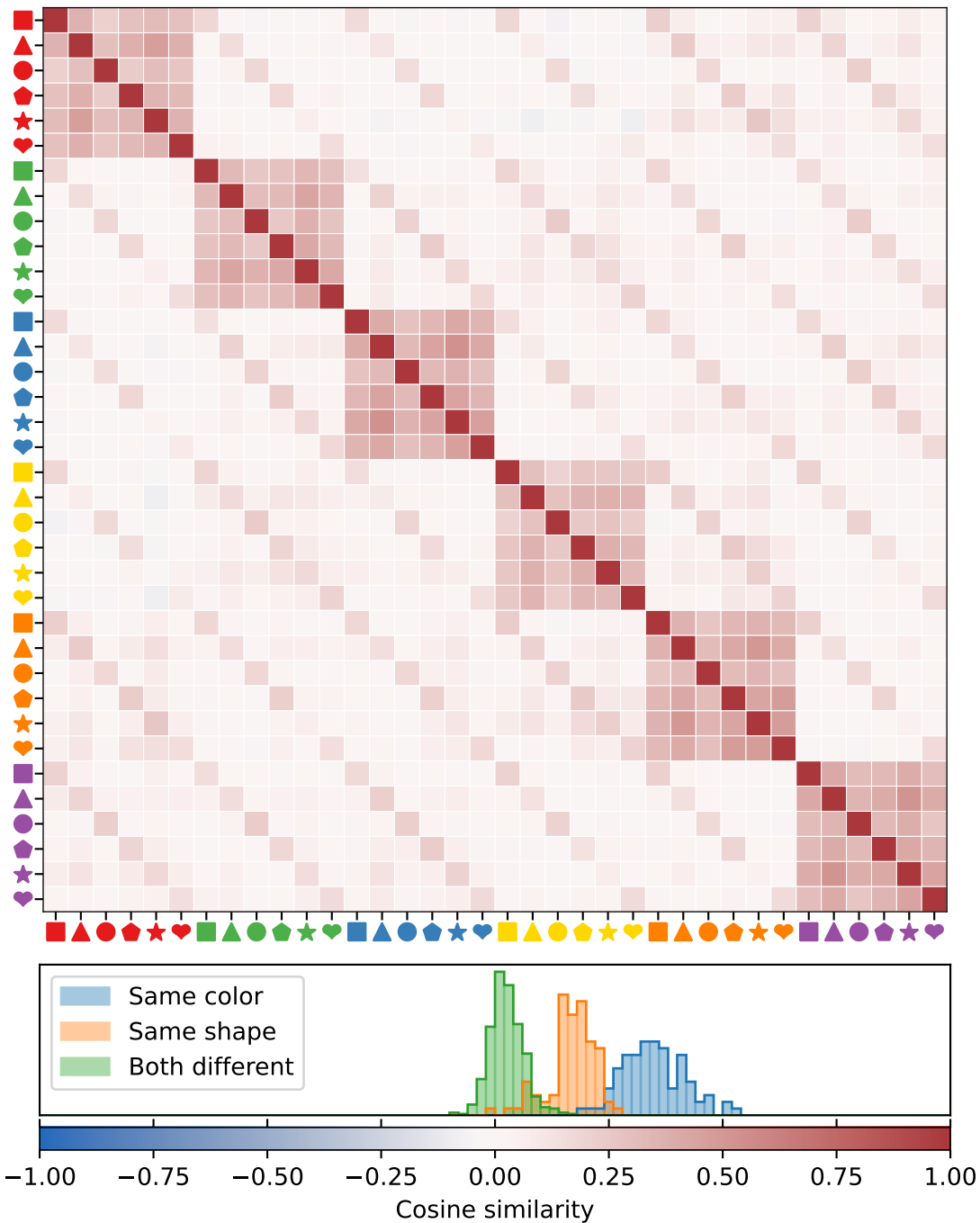
Gemma 3 12B - Probe-Based (Raw) Concept Vectors
