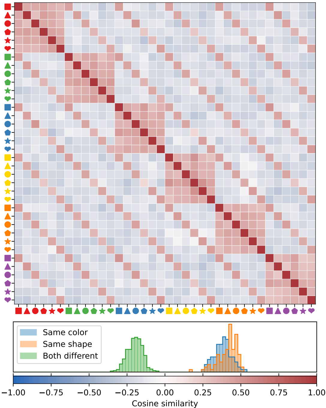
InternVL 2.5 8B - Probe-Based (PCA) Concept Vectors
