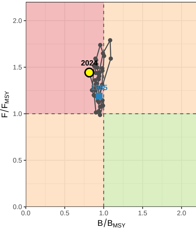
Kobe Plot: 1985 Constant M
