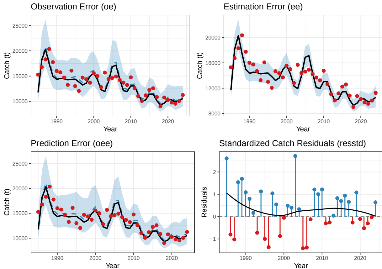
Figure 6: Aggregated catch diagnostics for the Constant M candidate run, detailing the separated variance components (observation, estimation, and prediction errors) and the standardized aggregated residuals.
