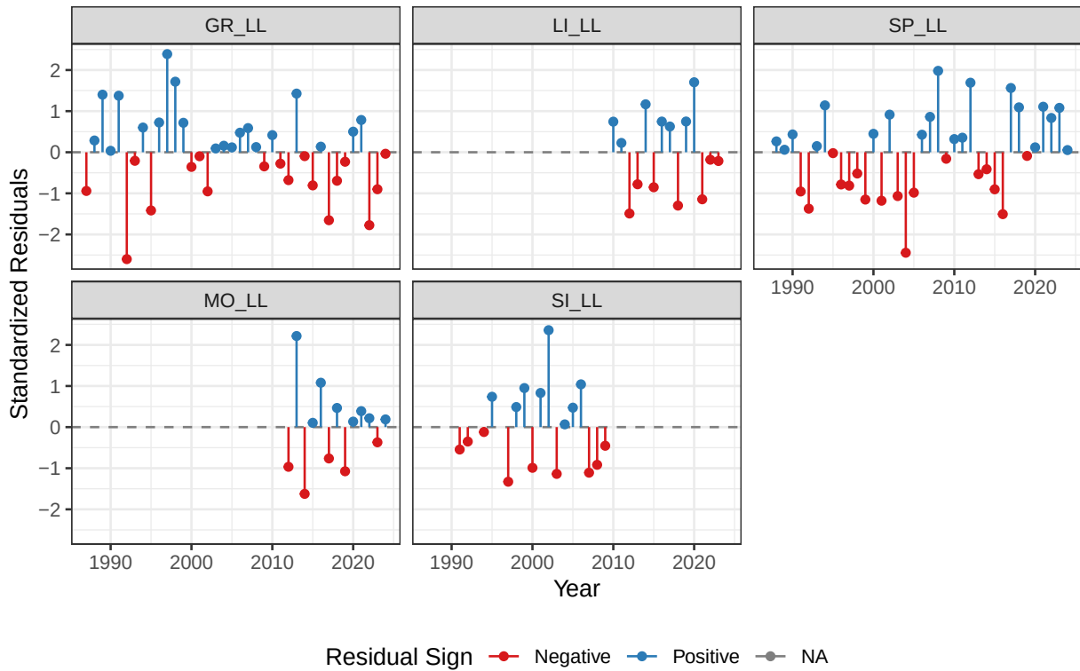
Figure 5: Standardized residuals for each CPUE index (Constant M).
