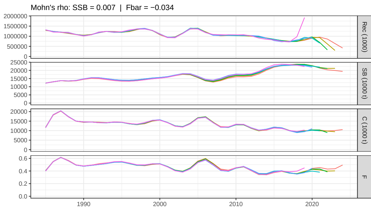
Figure 7: Retrospective analysis (5 peels) for the Constant M candidate run.
