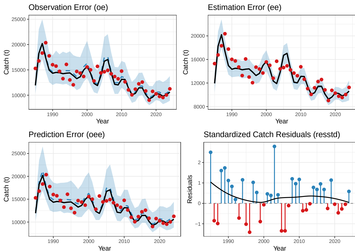
Figure 10: Aggregated catch diagnostics for the Lorenzen M candidate run, detailing the separated variance components (observation, estimation, and prediction errors) and the standardized aggregated residuals.
