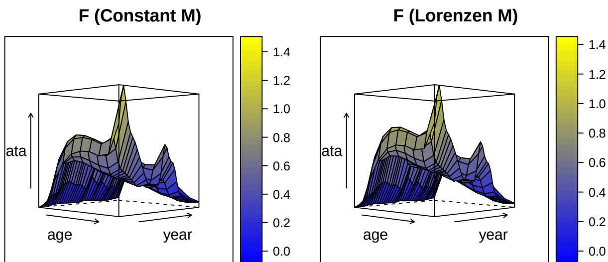
Figure 3: Fishing mortality at age over time (selectivity surface) for both candidate runs.
