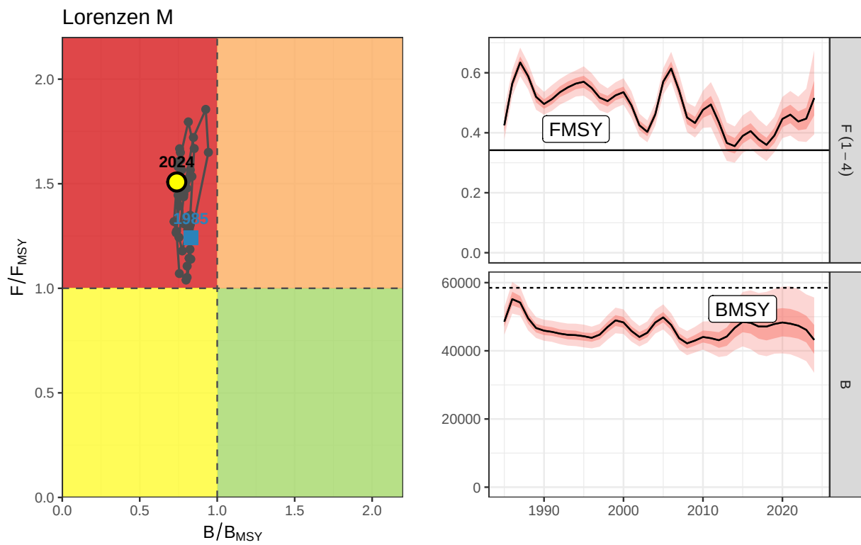
Figure 12: Kobe phase plot for the Lorenzen M and trajectories of SSB, F and B.
