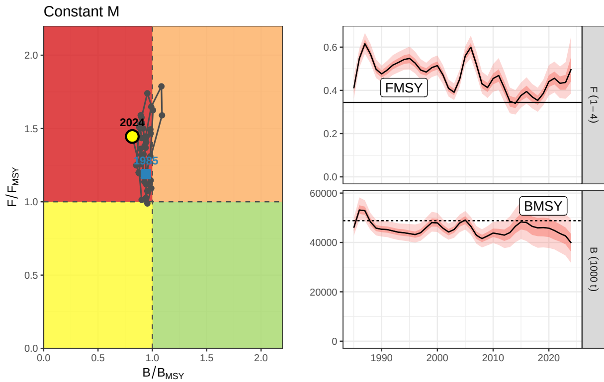
Figure 11: Kobe phase plot for the Constant M and trajectories of SSB, F and B.
