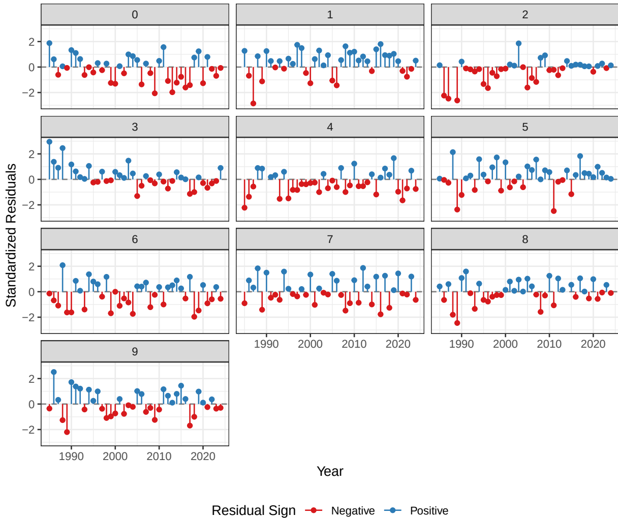
Figure 4: Standardized log-residuals of catch-at-age for the Constant M candidate run.
