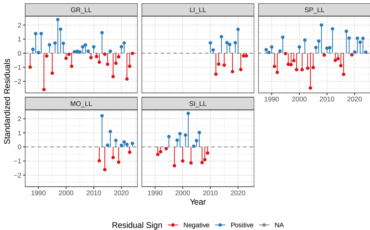
Figure 9: Standardized residuals for each CPUE index (Lorenzen M).
