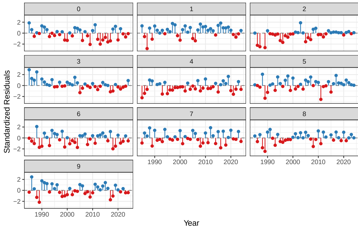
Figure 8: Standardized log-residuals of catch-at-age for the Lorenzen M candidate run.
