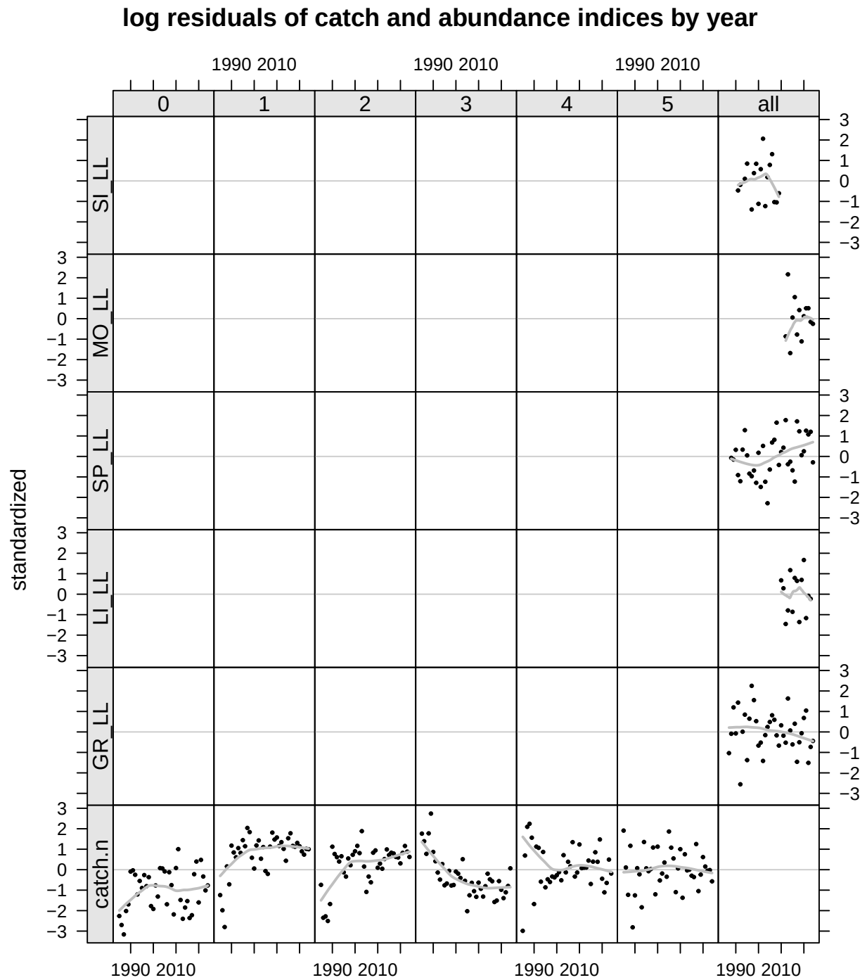
Figure 6: Standardized residuals of the 2026 updated a4a fit for the CPUE indices and catch-at-age.
