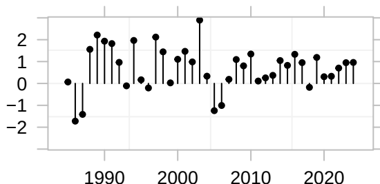
Standardized residuals
