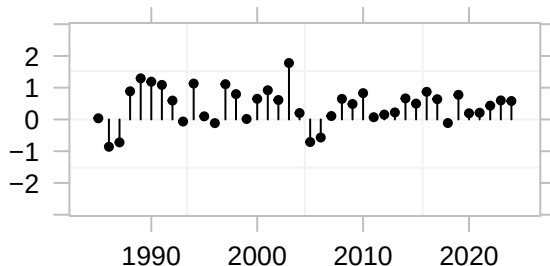
Pearson residuals
