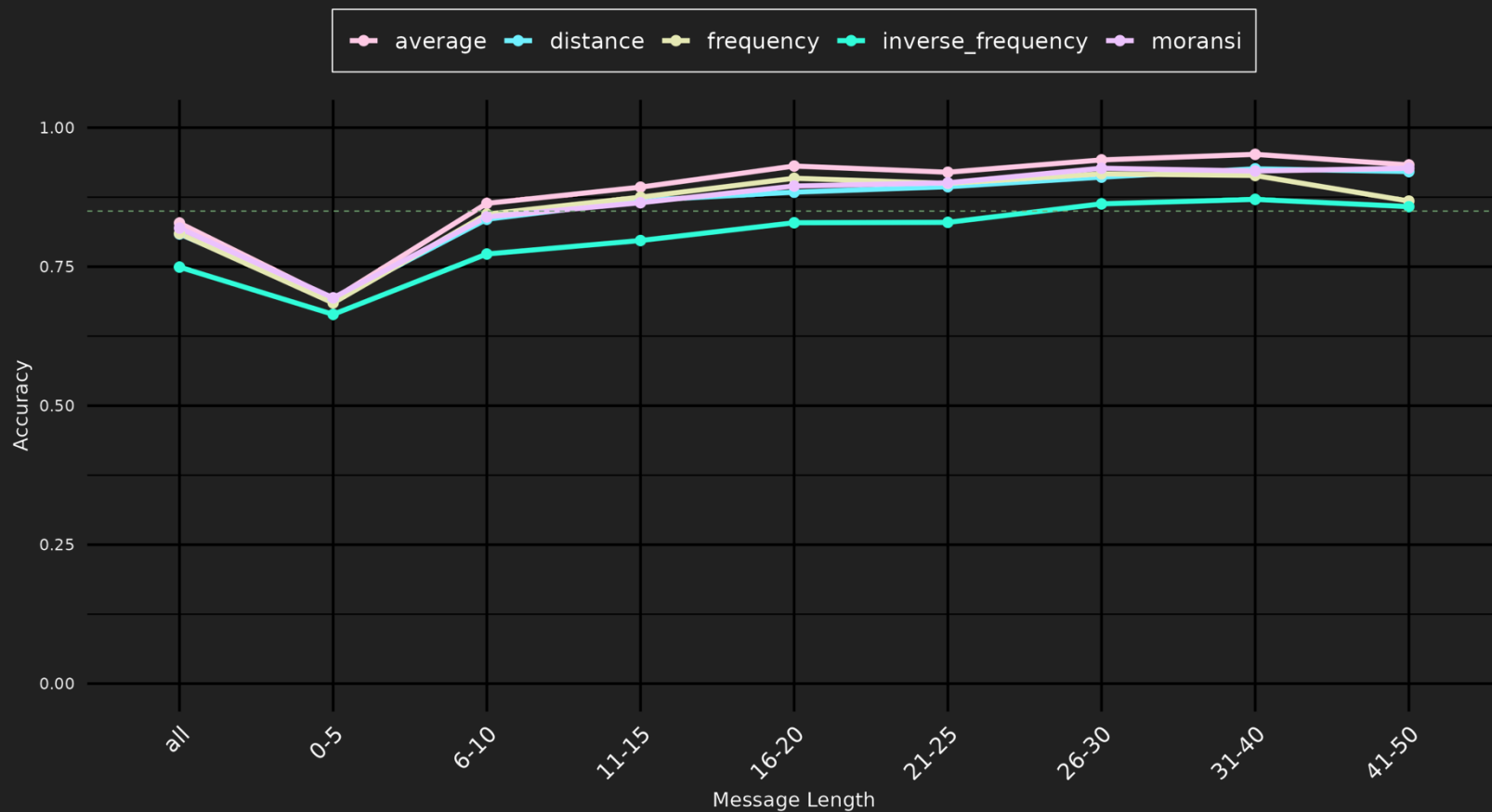
Country Accuracy given Message Length
