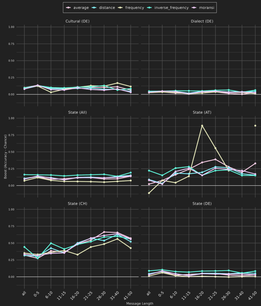
Region Accuracy Boost over Baseline by Message Length
