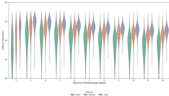
Figure 13: Latency vs. Max Peer Degree at BLE 1M PHY Range
