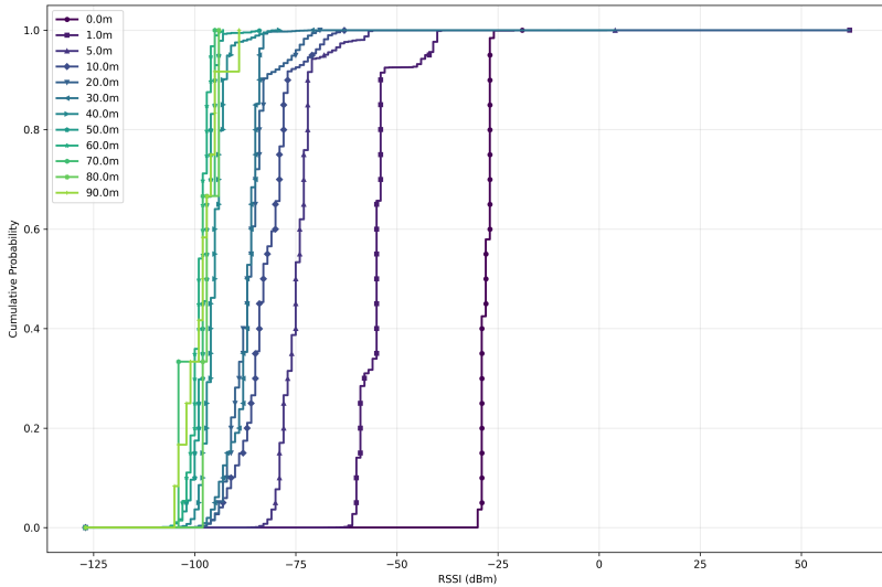
Figure 8: RSSI CDF
