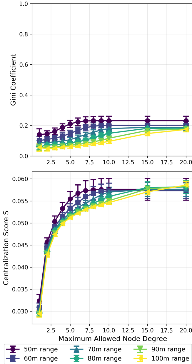
Figure 8: Centralization vs. max node degree - inter-cluster communication
