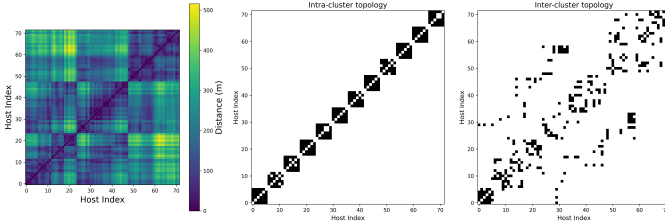
Figure 6: Topology and distance metrics for communication radius 100m, constrained maximum node degree 5
