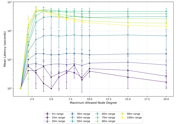
Figure 7: Latency vs. max node degree - inter-cluster communication
