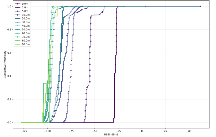
Figure 4: RSSI CDF
