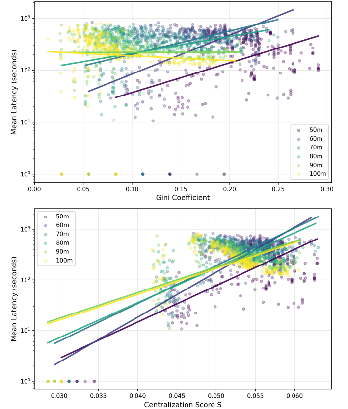
Figure 8: Latency vs. Centralization - inter-cluster communication
