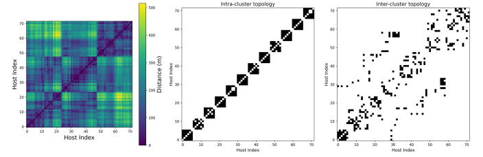
Figure 7: Topology and distance metrics for communication radius 100m, constrained maximum node degree 5
