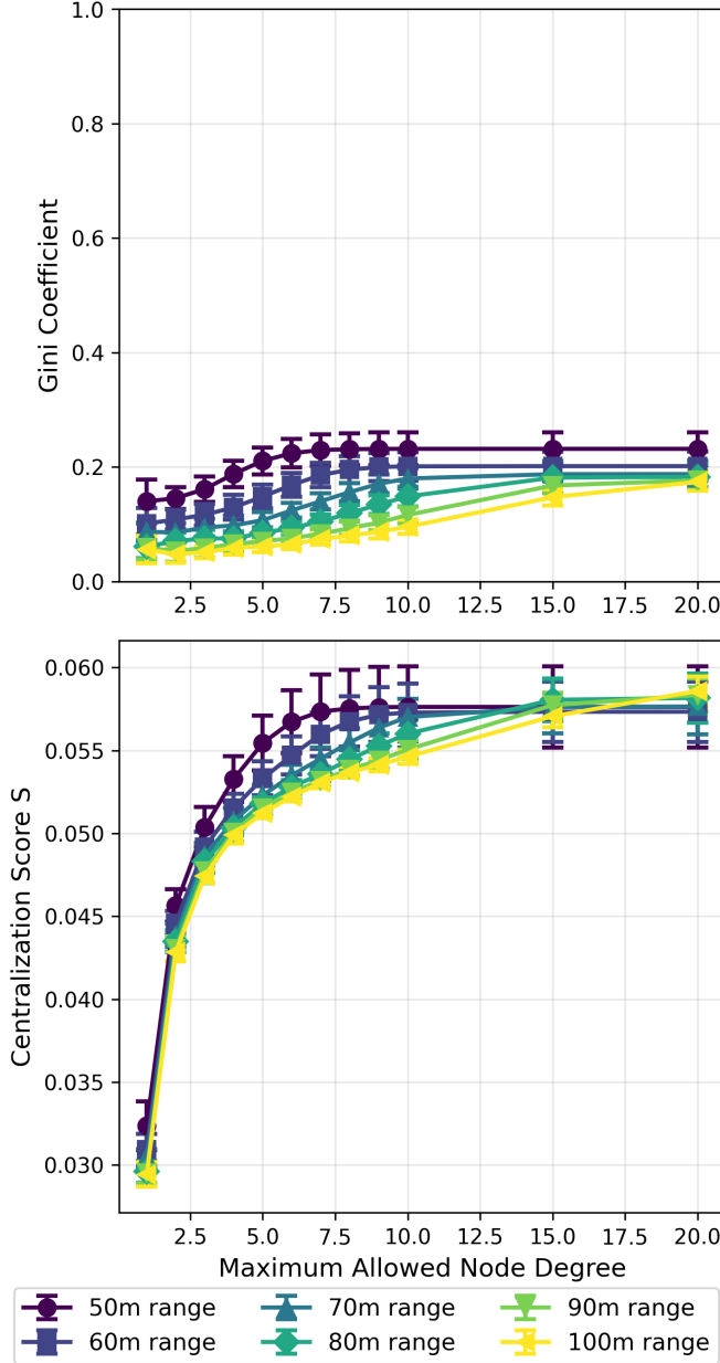
Figure 9: Centralization vs. max node degree - inter-cluster communication
