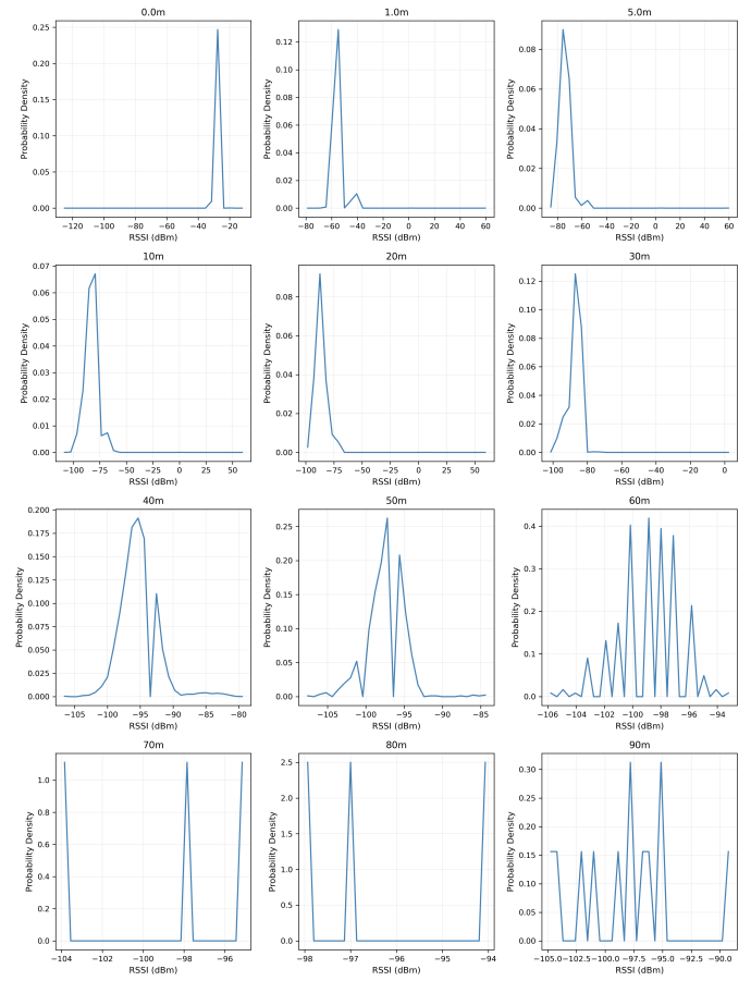
Figure 11: RSSI PDF
