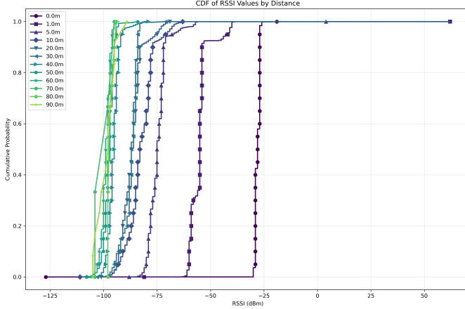
Figure 2: RSSI CDF
