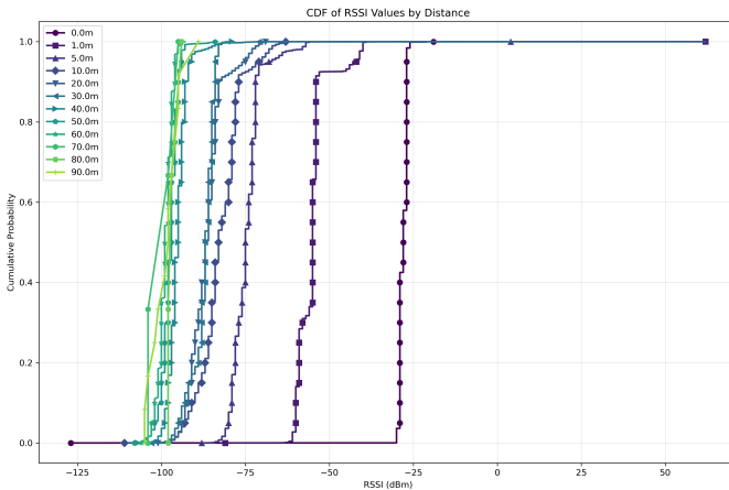
Figure 4: RSSI CDF
