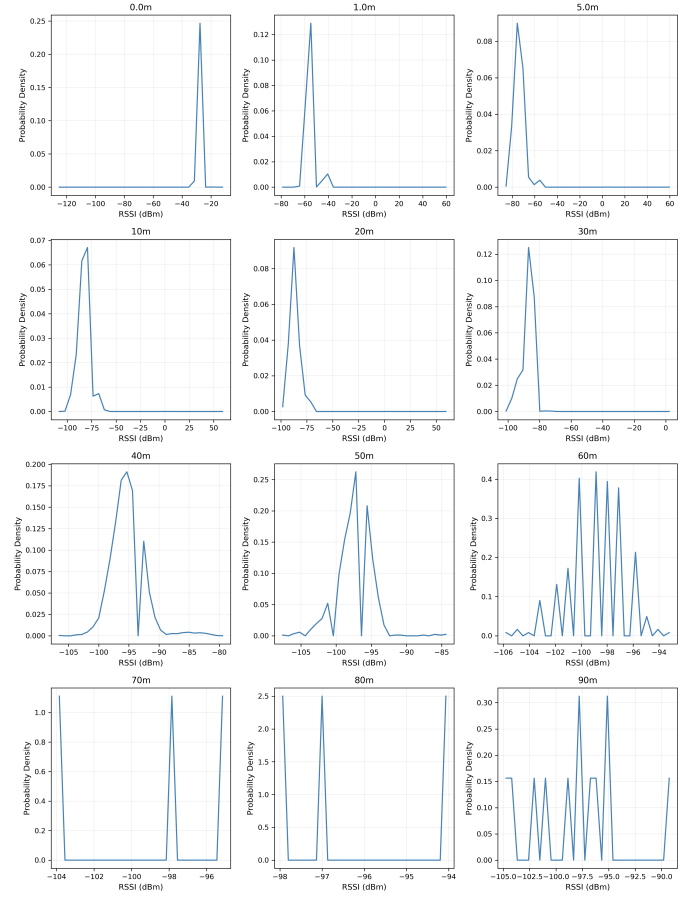
Figure 10: RSSI PDF
