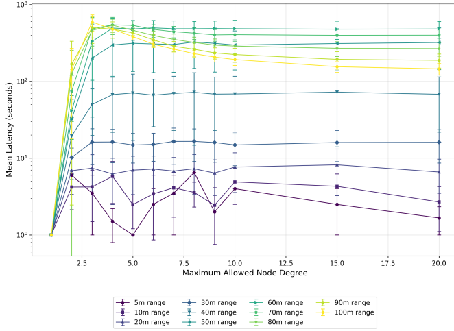
Figure 7: Latency vs. max node degree - inter-cluster communication
