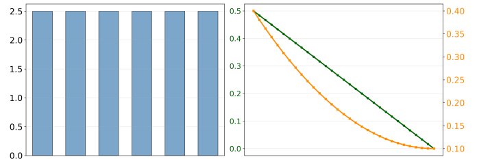
Figure 2: Dense topology
