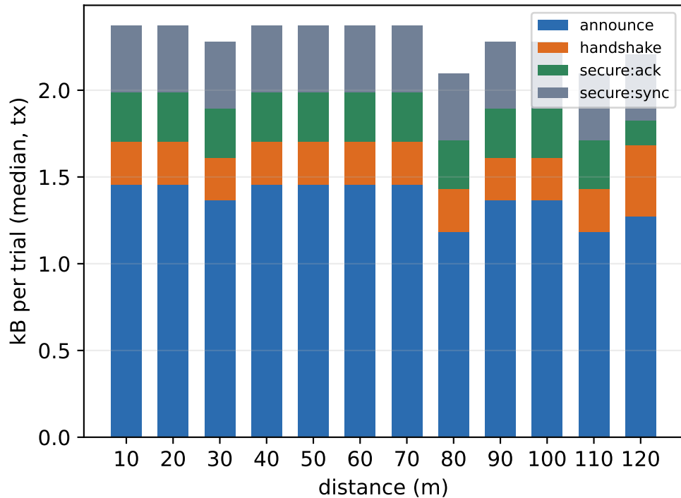
Control plane on the wire
