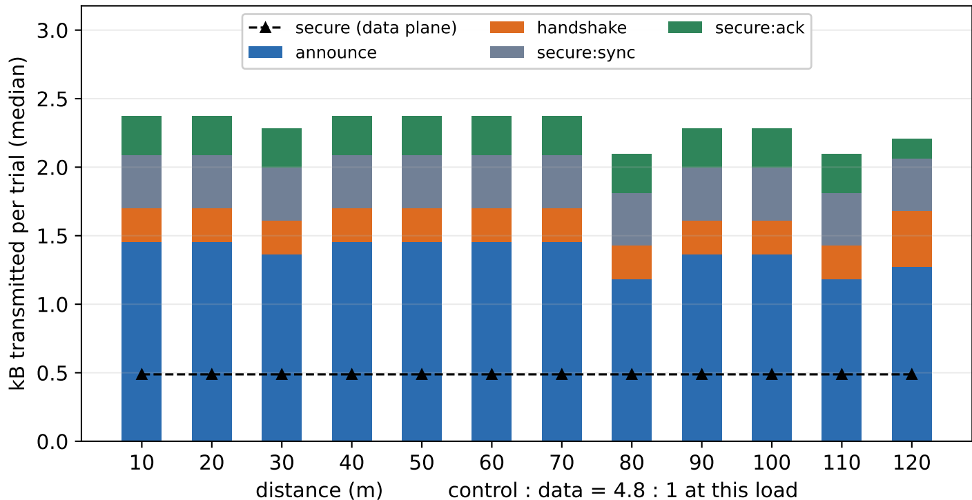
Control plane on the wire, by packet class
