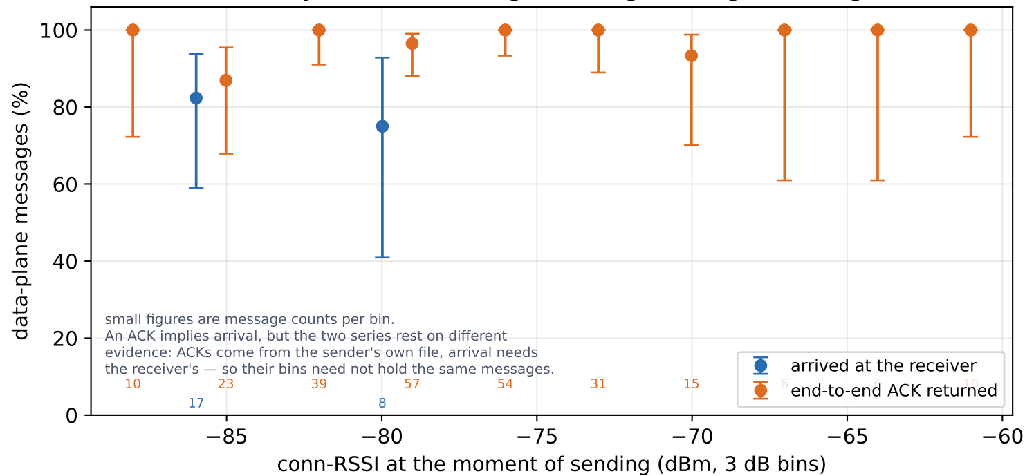
Delivery and acknowledgement against signal strength
