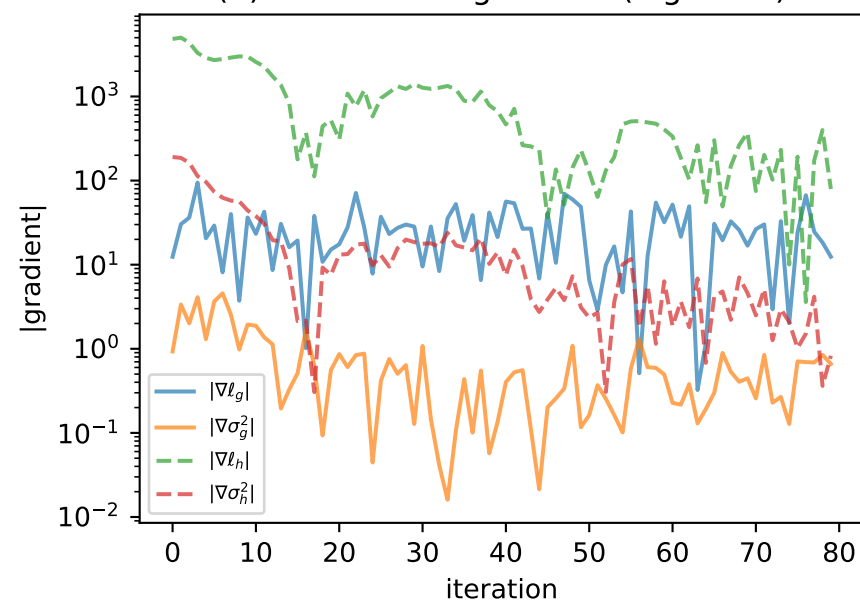
(n) Gradient magnitudes (log scale)
