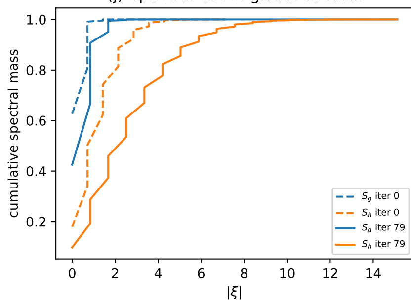
(j) Spectral CDFs: global vs local
