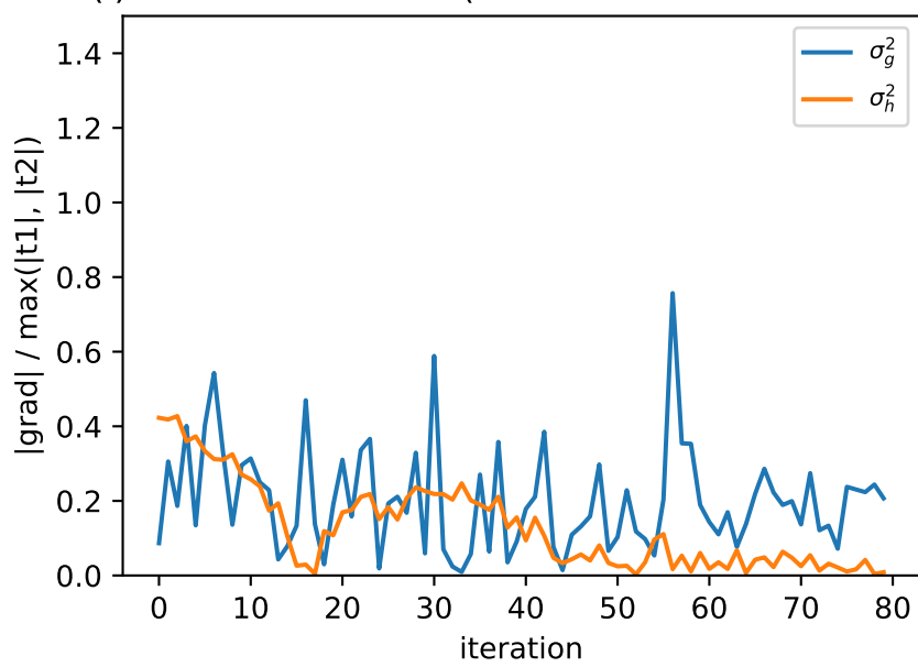
(l) Cancellation ratio (lower = more cancellation)
