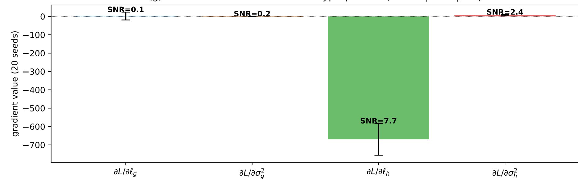
(g) Gradient mean \pm std at TRUE hyperparams (SNR = |mean|/std)
