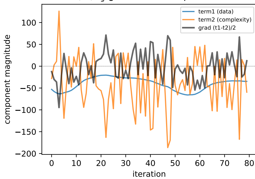
(m) \ell_g gradient decomposition
