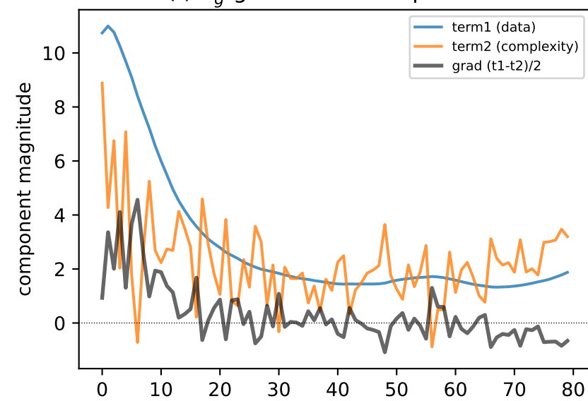
(f) \sigma_g^2 gradient decomposition
