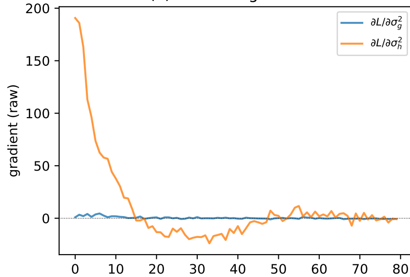
(e) Variance gradients
