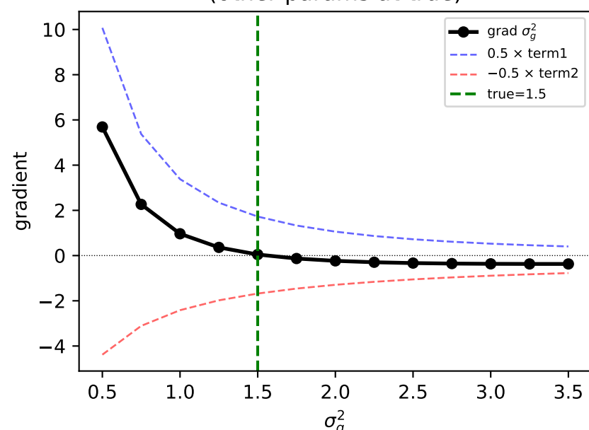
(k) \partial L / \partial \sigma_g^2 landscape (other params at true)
