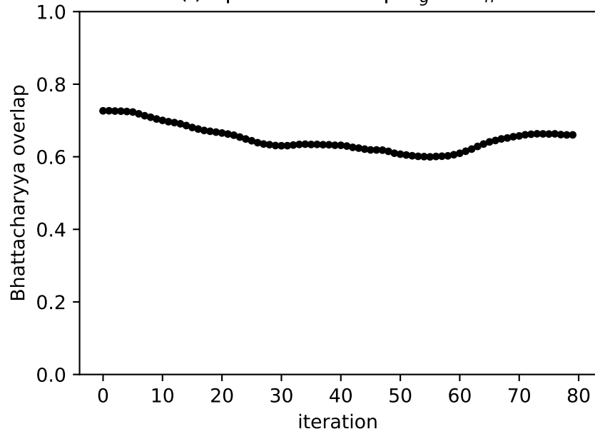
(i) Spectral overlap S_g vs S_h
