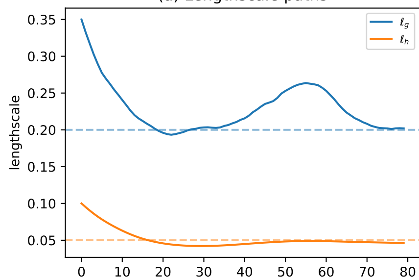
(a) Lengthscale paths
