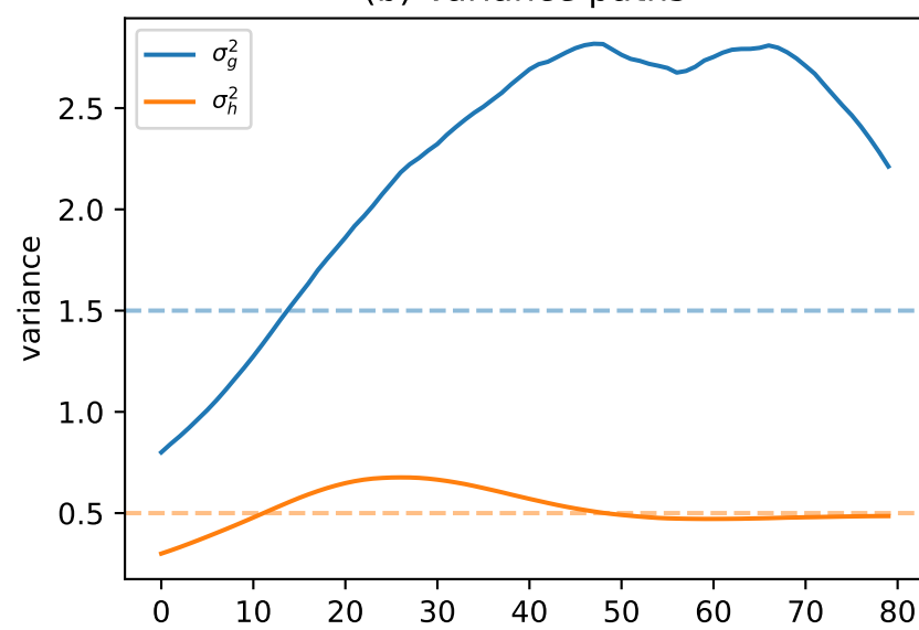
(b) Variance paths
