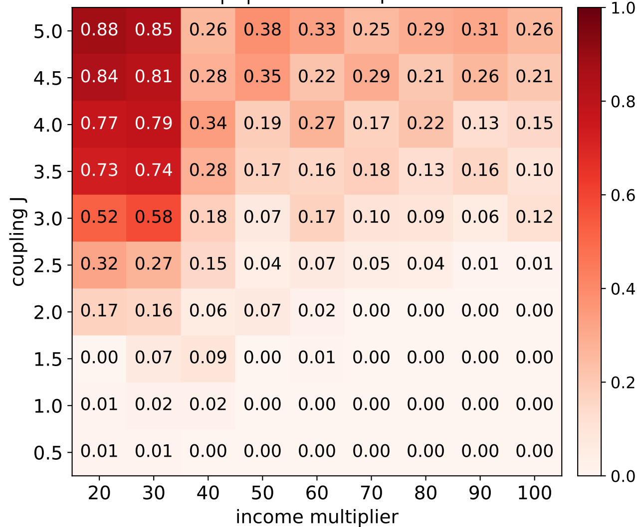
P(rigidity collapse) |m|>0.9 at collapse
