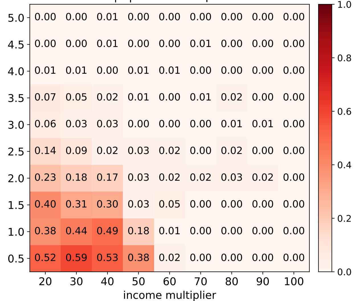
P(fragmentation collapse) |m|<0.3 at collapse
