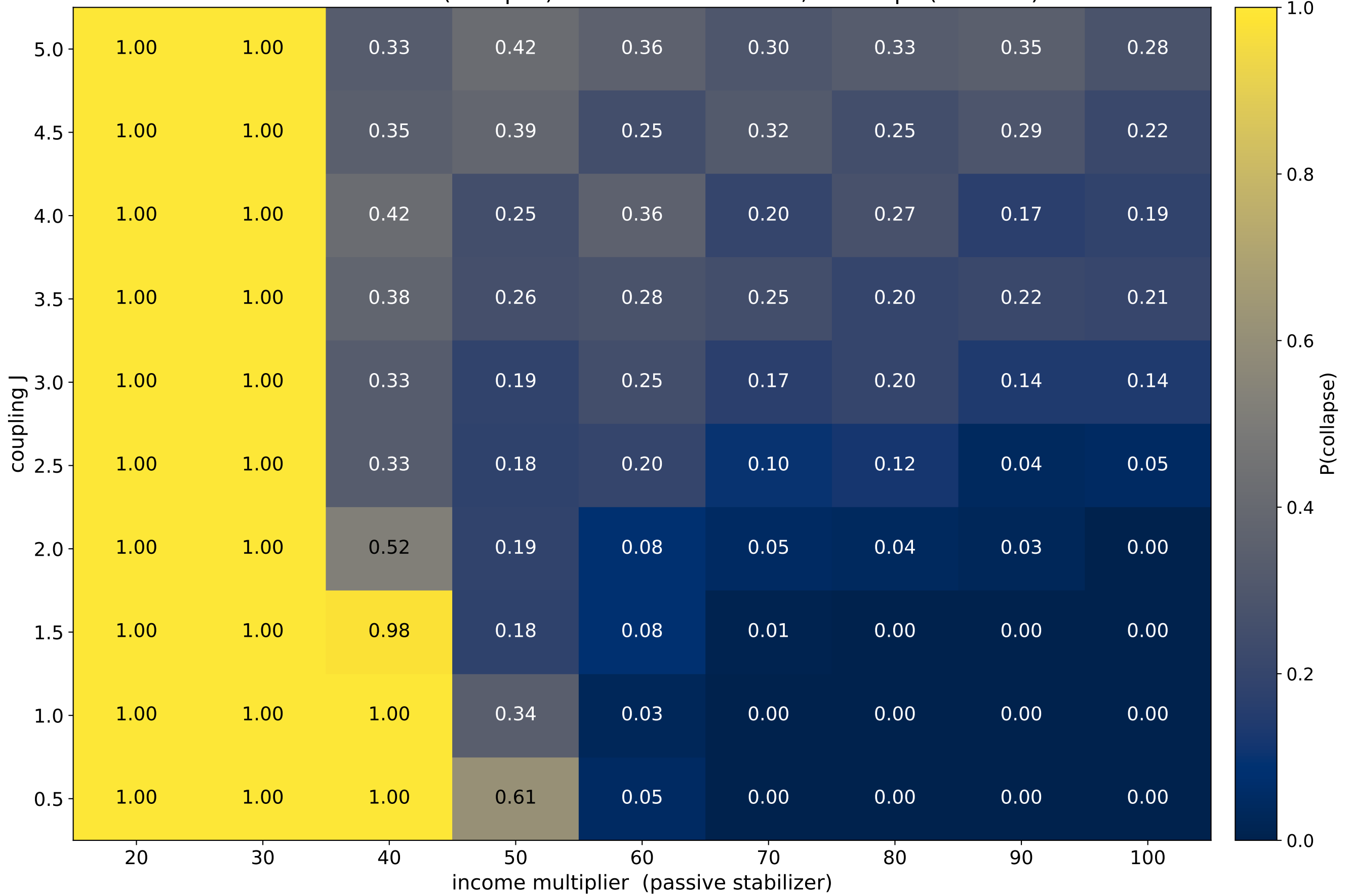
Minimal model: P(collapse) over 100 seeds × 20,000 steps (dt=0.05)
