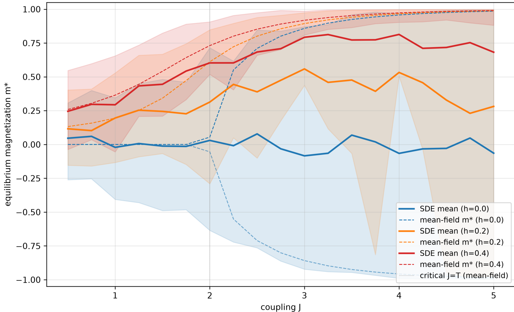
Level 0 — Pure CW SDE: equilibrium m vs J at fixed h high- |m| ordered regime emerges for J > T regardless of stabilizer
