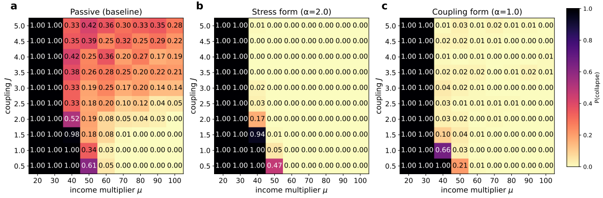
Figure 2: Matched-seed stabilizer contrast . Matched-seed P(collapse) over (J, \mu) : wealth-fed baseline h = 2 \cdot (W/500) (a, left), stress form ( \alpha = 2.0 , b, center), coupling form ( \alpha = 1.0 , c, right). The baseline reproduces the high- J residual (band-mean 0.23 at \mu = 100 ); the stress and coupling forms show P(\text{collapse}) = 0.00 across J \geq 4.0 at \mu = 100 (95% upper bound 0.03 per 100-seed cell) and \leq 0.01 respectively. 9,000 runs/condition, dt = 0.05 . The contrast stands as a measurement. A pre-registered magnitude-matched control (E2; Results; Supplementary Section S5.6) shows that matching a stabilizer’s full-trajectory delivered mean does not reproduce its outcome: a pure constant carrying the stress form’s full-trajectory delivered mean collapses far less than the stress form at an informative operating point (0.000 vs 0.281, REFUTED in all three cells). The contrast is reported here as a measurement, not as evidence for a single delivered-amplitude cause.
