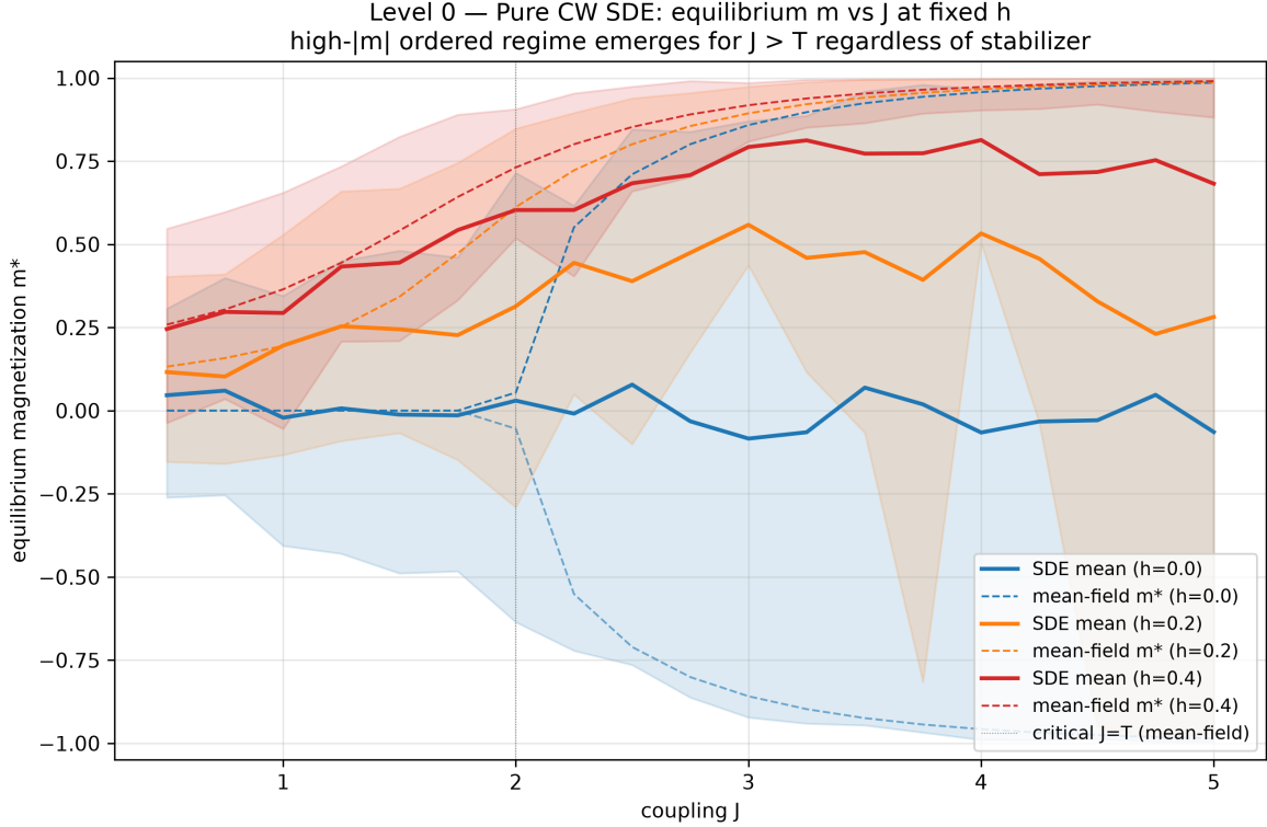
Supplementary Figure S1: Mean-field equilibrium curves for the bare Curie–Weiss SDE (Level 0). The figure shows the long-time mean of independent SDE trajectories at each (J, h) cell, with h held fixed at three values ( h \in \{0.0, 0.2, 0.4\} ) and J swept across \{0.5, \dots, 5.0\} . Dashed curves are the analytical mean-field fixed points obtained by solving Equation S1 numerically; solid colored curves are the SDE long-time means with shaded bands showing the interquartile range across seeds. For h > 0 (orange and red), the SDE cross-seed mean tracks the upper mean-field branch at low coupling but falls increasingly below it as J rises (e.g. at h = 0.2 the mean is \approx 0.23 against an upper branch \approx 0.99 by J \approx 4.75 ). This is not a breakdown of the mean-field description but the finite-noise residual-selection effect central to this paper: a fraction of seeds are noise-selected onto the lower ( -m ) branch (the lower quartile reaches \approx -0.95 at high J while the upper quartile continues to track the upper branch), dragging the cross-seed average down. For h = 0 (blue), the SDE mean fluctuates around zero — an expected finite-sample effect under spontaneous symmetry breaking, where individual seeds lock onto either the +1 or -1 branch and the cross-seed average cancels — while the mean-field curves plotted show both symmetric branches. This validates the analytical backbone of Proposition 1: the mean-field free-energy structure used to derive the h/J scaling in §S2 is the correct effective description of the bare SDE in the absence of the wealth–field coupling, modulo the finite-sample symmetry-breaking caveat at h = 0 which does not affect Proposition 1 (which applies for h \neq 0 ). Source file: simulation/results/ablation/level0_equilibrium_curves.png ; rendered here as Supplementary Figure S1, manuscript/arxiv/figures/figS1.png . The multiplicative noise term \xi\sqrt{1-m^2} vanishes at the saturated branches and does not distort the branch structure (the two wells remain at \approx \pm 1 ); the high- J downward drift of the cross-seed mean is the §S2.7 residual-selection effect, not a numerical artifact of the dt = 0.1 integration or the clipping rule m \in [-1 + \varepsilon, 1 - \varepsilon] employed in the integrator.
