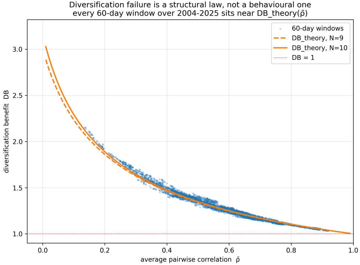
Figure S2: Structural diversification failure (supporting the “Empirical setting” Results subsection). Diversification benefit DB versus average pairwise correlation \rho across 5,414 sixty-day rolling windows of nine US sector ETFs (XLRE appended on its 2015-10-08 inception, yielding a 10-sector panel post-2015), 30 March 2004 – 30 December 2025. The theoretical structural curve DB(\rho, N) = 1 / \sqrt{(1/N + (1 - 1/N) \rho)} is overlaid; mean absolute error of empirical points against the curve is 0.016, with maximum deviation 0.100. Spearman \rho(\rho, DB) = -0.993 ( p < 10^{-15} ). Named crisis episodes (peak \rho , minimum DB during the episode): GFC 2008 (0.83, 1.08); Eurozone crisis 2010–12 (0.92, 1.03); China devaluation 2015 (0.80, 1.10); COVID-19 selloff 2020 (0.92, 1.04); inflation shock 2022 (0.74, 1.16). Each crisis sits on the predicted curve. Source file: empirical/figures/diversification_failure_scatter.png .
