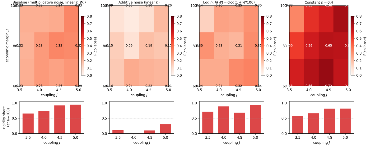
Figure S4: Sensitivity sweep — noise prescription and h(W) form (supporting §S5.1). Top row: P(\text{collapse}) heatmap over the high- J band ( J \in \{3.5, 4, 4.5, 5\} ) \times protective-margin band ( \mu \in \{60, 80, 100\} ) for four model variants — baseline (multiplicative noise \xi\sqrt{1-m^2} , linear h(W) = 2(W/500) ), additive noise (constant \xi , linear h ), logarithmic h(W) = 0.577 \cdot \log(1 + W/100) , and constant h = 0.4 . Bottom row: rigidity share at \mu = 100 across the J range for each variant. Headline cell ( J = 5, \mu = 100 ): baseline 0.33, additive 0.20, log h 0.30, constant h 0.70. The qualitative residual is robust to log-vs-linear h ; constant h is substantially worse, ruling out the baseline as a tuned best-case; under additive noise the residual persists but rigidity-typed dominance falls ( 0.94 \rightarrow 0.30 ), confirming the h/J^2 landscape result is multiplicative-noise-specific while the asymmetry itself is not. 4,800 runs total (100 seeds per cell \times 12 cells \times 4 variants). Source files: simulation/scripts/sensitivity_sweep.py , simulation/results/sensitivity/figure_s4_sensitivity_sweep.png .
