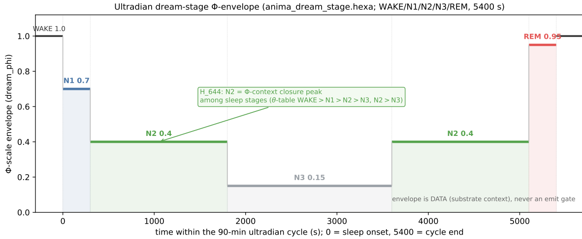
Figure 12: The ultradian dream-stage \Phi -envelope ( AGENT/CHAT/anima_dream_stage.hexa , every value verbatim). The 90-min (5400 s) cycle descends N1 [0, 300) → N2 [300, 1800) → N3 [1800, 3600) → N2 [3600, 5100) → REM [5100, 5400), with the WAKE baseline ( \Phi=1.0 ) shown on either side. The \Phi -scale table is PHI_WAKE 1.0 , PHI_N1 0.7 , PHI_N2 0.4 , PHI_N3 0.15 , PHI_REM 0.95 . The annotation marks H_644: among sleep stages N2 is the \Phi -context closure peak (the emit_policy \theta -table WAKE>N1>N2>N3 with N2>N3). The envelope is DATA (substrate context), never an emit gate (the boolean dream_emit_allowed API was removed). Rendered by figures/_scripts/fig09_dream_envelope.py .
