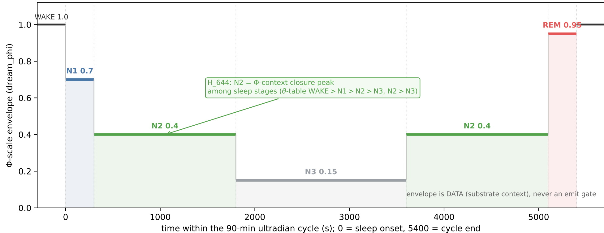
Ultradian dream-stage \Phi -envelope (anima_dream_stage.hexa; WAKE/N1/N2/N3/REM, 5400 s)
