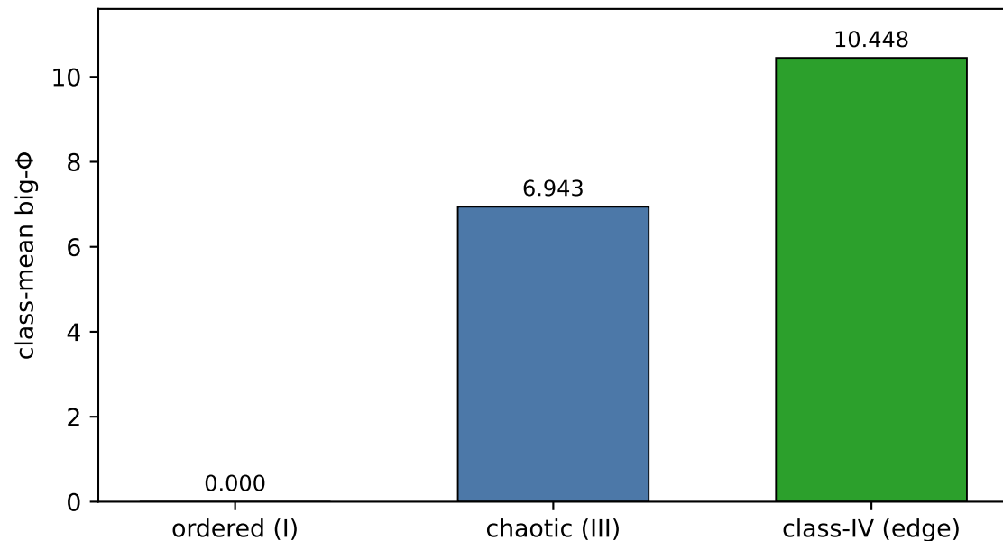
(b) edge-of-chaos \Phi -peak (H\_285) ordered < chaotic < edge
