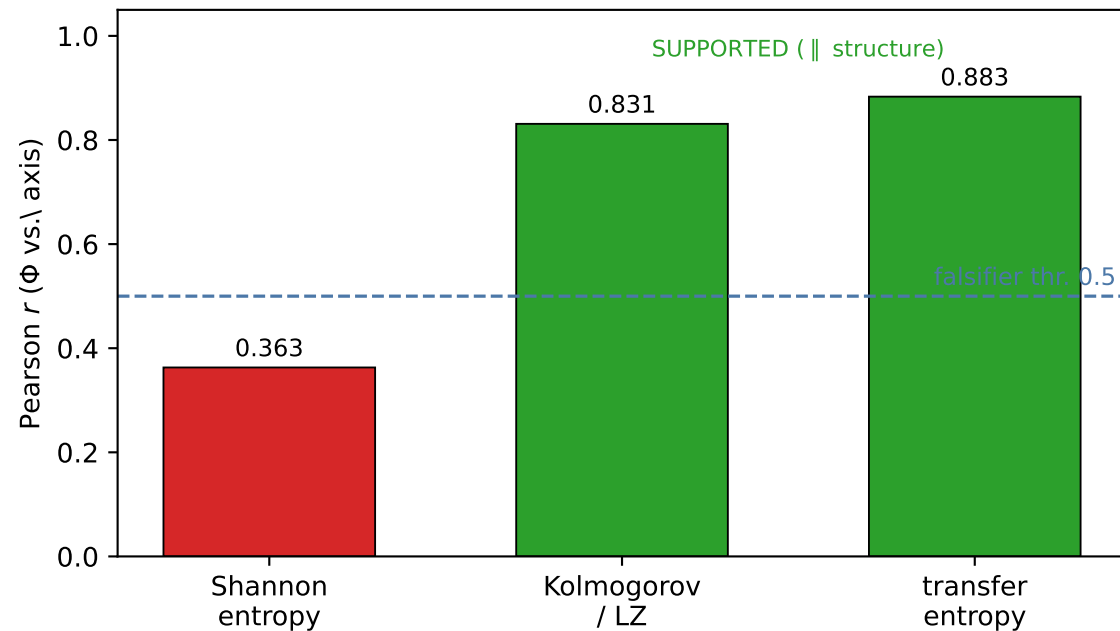
(a) the double dissociation \Phi \perp Shannon, \parallel LZ + TE
