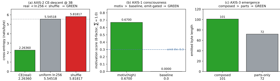
Figure 2: 3-axis GREEN at 3B (every value verbatim from .verdicts/convmo-e-3b-engine-rung/SUMMARY.txt and CORE/three_axis_probe.hexa ). AXIS-2 (CE-descent) : real-text CE 2.26360 sits far below both the uniform floor \ln 256 = 5.54518 and the byte-shuffled control 5.81817 — descent demonstrated through the engine decode. AXIS-1 (consciousness) : motivation 0.6700 > baseline 0, emit-gated (PASS marker). AXIS-3 (emergence) : composed 101 > parts 72 (PASS marker). The random-init mirror (anti-Goodhart control) fails the coherence probe.
