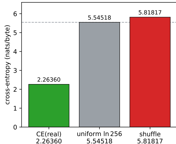
(a) AXIS-2 CE-descent @ 3B real < \ln 256 < \text{shuffle} \Rightarrow \text{GREEN}
