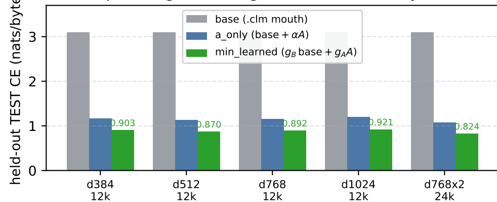
(a) per-rung CE: min-gate HOLDS at every scale
