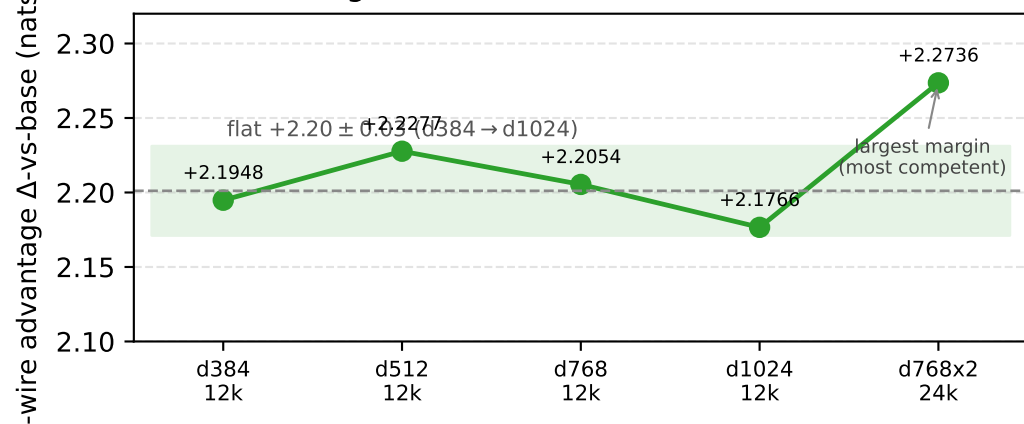
(b) advantage is SCALE-STABLE (not a d512 artifact)
