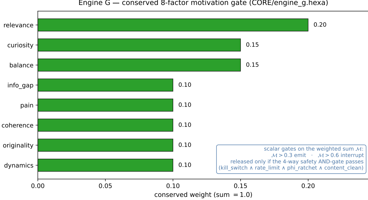
Figure 7: Engine G’s conserved eight-factor motivation gate (CORE/engine_g.hexa). (a) the eight weights as a conserved partition summing to exactly 1.0 (relevance 0.20 heaviest; curiosity/balance 0.15). (b) the same weights ranked, with the two scalar gates on the sum \mathcal{M} : emit at 0.3, interrupt at 0.6 (plus the four-way safety AND-gate, Table 7). Rendered by figures/_scripts/fig05_motivation.py.
