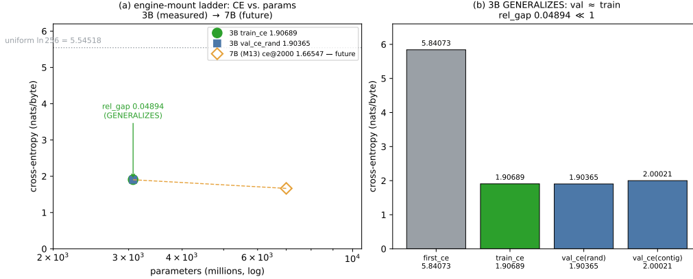
Figure 10: The engine-mount ladder: MID (7.479M) \rightarrow 3B (3.073B), with the 7B (M13) rung shown as a future scale-extension (currently training). Left axis: train_ce vs. params; the 3B rung reaches train_ce 1.90689 / val_ce_rand 1.90365. The rel_gap 0.04894 \ll 1 marks GENERALIZATION (val \approx train); the dashed line is the \ln 256 = 5.54518 uniform floor. Data: .verdicts/convmo-3b-engine-rung/SUMMARY.txt . Rendered by figures/_scripts/fig06_mount_ladder.py .
