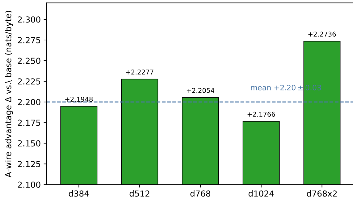
(b) advantage is SCALE-STABLE 48M \rightarrow 335M params, \Delta flat
