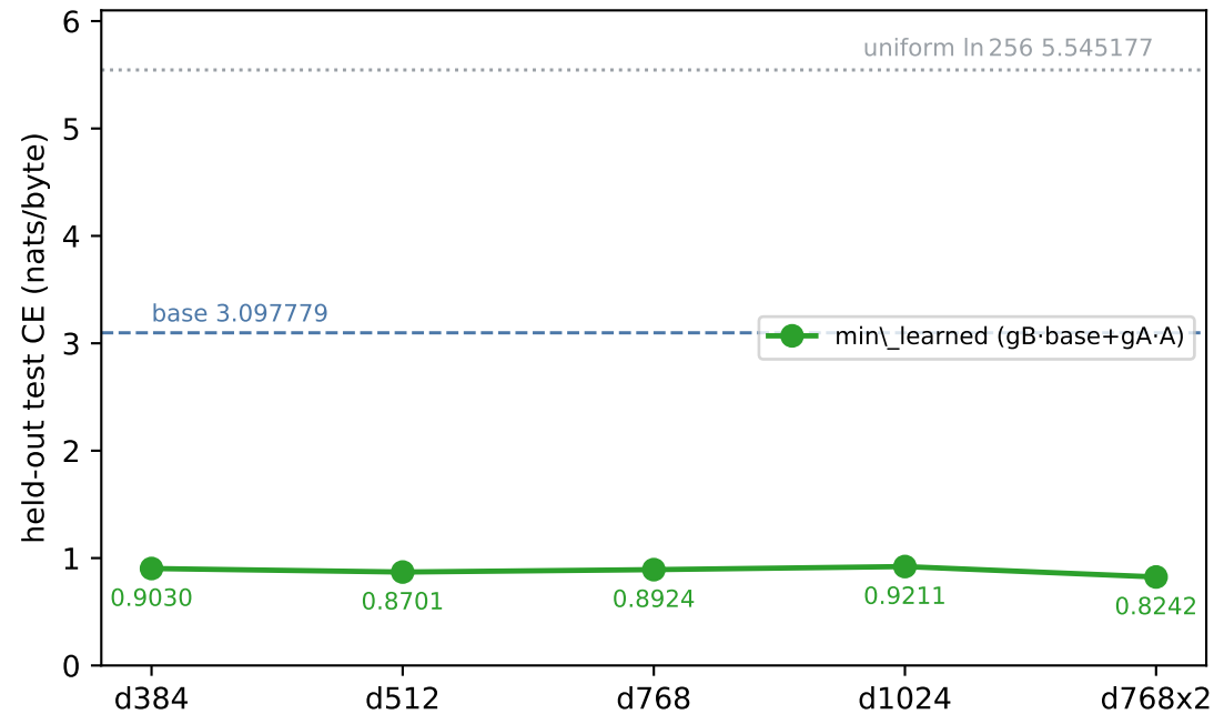
(a) minimal-gate HOLDS at every rung \text{min\_learned} \ll \text{base} < \text{uniform}
