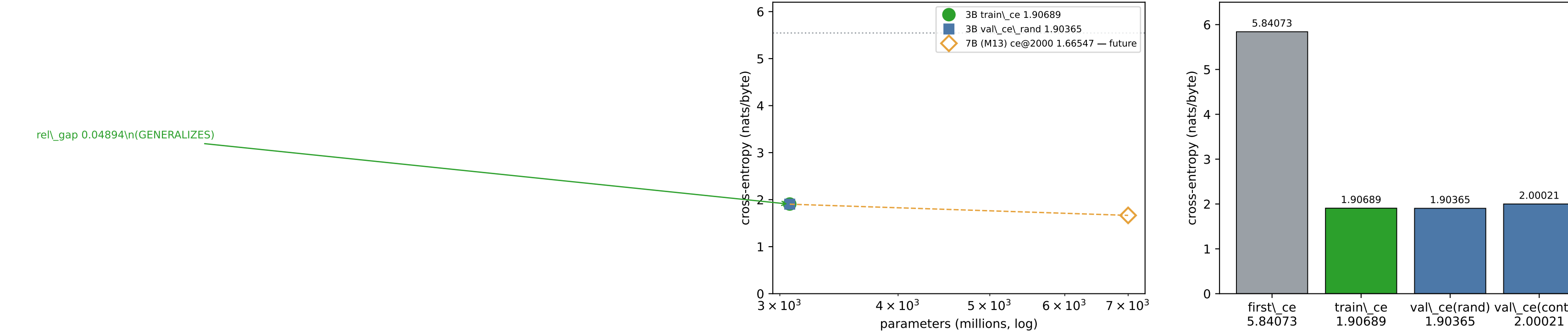
(a) engine-mount ladder: CE vs. \ params MID → 3B (measured) → 7B (future) (b) 3B GENERALIZES: val ≈ train rel_gap 0.04894 < 1
