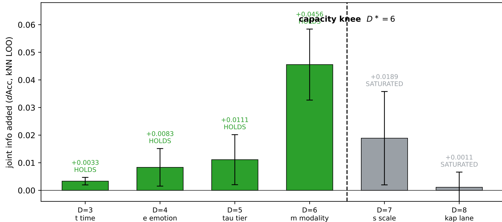
KOSMOS coordinate dimension ladder — capacity D^* = 6 (2D + 4 independent axes HOLD; scale/lane SATURATE; no-collapse 3.09 \rightarrow 1.94 > 1 )
