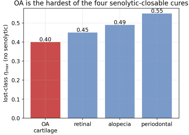
Figure 9: Lost-class restoration ceiling \eta_{\max} across the four senolytic-closable cures. OA (0.40) is the lowest, making it the hardest and the only triple-gated member.
