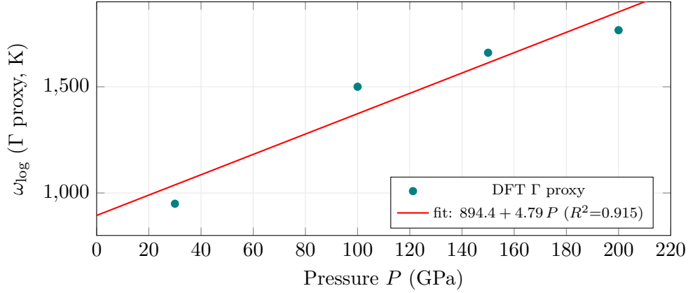
Figure 6: \text{H}_3\text{Br} \omega_{\log} versus pressure (Γ-point proxy). The positive slope +4.79 \text{ K GPa}^{-1} ( 9.6\times the F-N6-4 threshold) confirms the \omega_{\log} bottleneck is pressure-responsive; every point is dynamically stable (zero imaginary modes). The absolute values are a Γ-only proxy (Limitations); the slope and monotone trend are robust.
