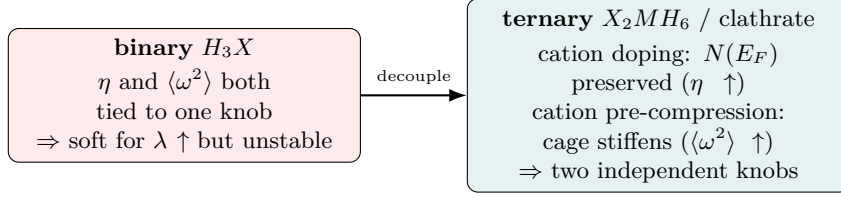
Figure 5: The cation-decoupling hypothesis. In binary hydrides a single knob ( \langle\omega^2\rangle ) controls both coupling and stability; a stuffed-cation phase can in principle move them independently. \text{CaH}_6 ( m = +0.5 , Apx. D) is the existence proof; the ambient X_2MH_6 octahedral instances tested here ( m < 0 , unstable) are not.
