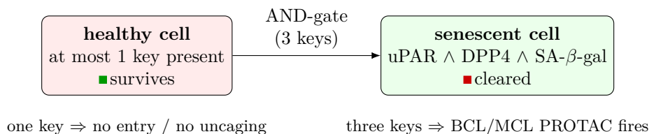
Figure 1: The SENOLYX-AG AND-gate. Selectivity is multiplicative across three orthogonal recognition axes; the warhead is a pan-senescent dependency (BCL-x L /MCL-1), not an affinity-maximized binder.
