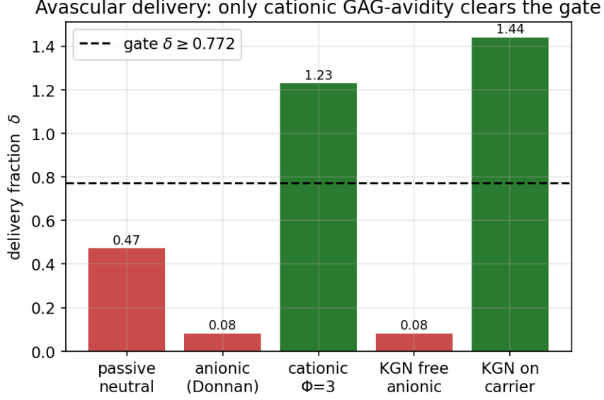
Figure 4: Delivery lever \delta from the 1-D transient reaction–diffusion model into 2 mm cartilage. Passive (0.472) and anionic (0.081) BLOCK against the 0.772 gate line; cationic GAG-avid (1.23) and carrier-conjugated KGN (1.44) PASS. Free anionic KGN (0.081) is Donnan-excluded.
