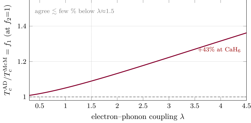
Figure 4: The McMillan→Allen–Dynes correction ratio f_1 vs \lambda ( \mu^* = 0.10 , f_2=1 ). The ratio is the formal statement of the divergence charted in Fig. ?? : \approx 1 in the conventional regime, growing to +43% by the strong-coupling hydride end. This is why the candidate slate of Appendix ?? is ranked by Allen–Dynes, not McMillan.
