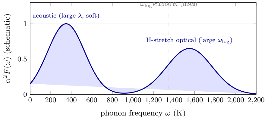
Figure 9: Schematic Eliashberg spectral function \alpha^2 F(\omega) for a hydride candidate. The soft acoustic band (metal sublattice) dominates \lambda via the 1/\omega weighting of Eq. (14); the stiff H-stretch optical band (light hydrogen) sets the high \omega_{\log} that lifts the T_c prefactor. The dotted line marks the h3cl \omega_{\log} \approx 1350 K. Shape is illustrative; the moments are the sourced numbers of Table 10.
