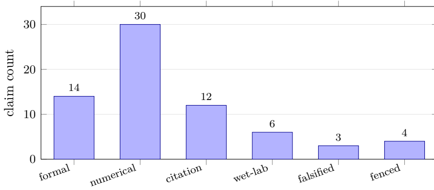
Figure 11: V4 tier distribution (Table 11). The closed/ numerical core (■ 14 + ■ 30 = 44) is the algorithm closure; the ■ 6 + ■ 3 are the honestly-preserved wet-lab deferrals and falsified negatives. This is the load-bearing honesty shape of the whole stack.
