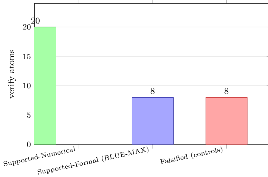
Figure 10: Verify-ledger tier distribution (companion/verify-ledger.json): 20 ■ SUPPORTED-NUMERICAL libm-class recomputes, 8 ■ SUPPORTED-FORMAL BLUE-MAX algebraic-root attestations, and 8 ■ FALSIFIED matched negative controls — 36 atoms total across 8 landing PRs. The controls are kept permanently: a negative control is evidence, never noise.
