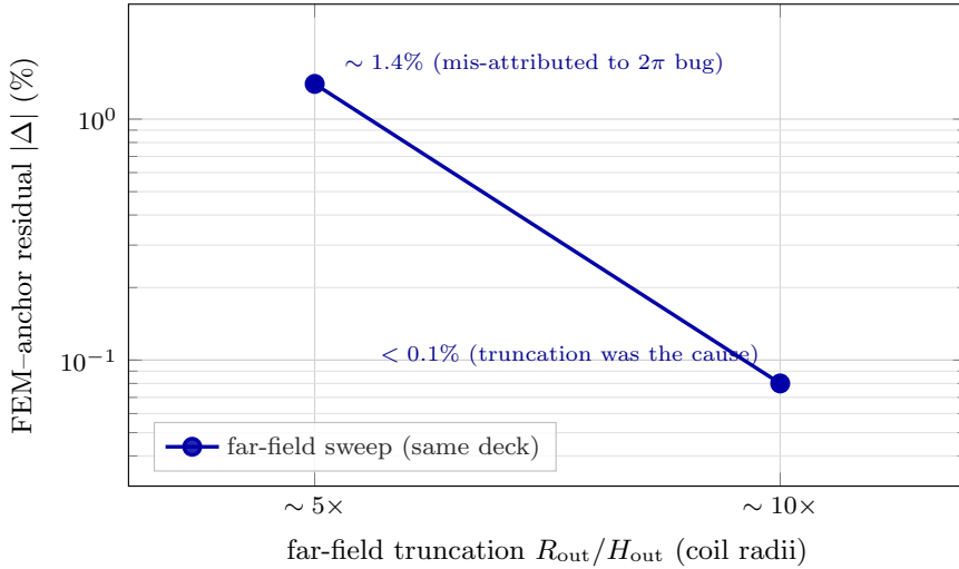
Figure 7: Far-field-truncation sweep (semilog- y ), the load-bearing methodological finding of this appendix. On the same deck and Jacobian, pushing the air-box outer boundary from R_{\text{out}}/H_{\text{out}} \approx 5\times to \approx 10\times the coil radius collapses the FEM-anchor residual from \sim 1.4\% to < 0.1\% — more than an order of magnitude. This proves the originally suspected 2\pi/\text{VolAxiSqu} units bug was a false diagnosis (Table 13): a correctly-formed 2\pi r measure fails loudly (integer-factor offset), while truncation fails quietly (smooth percent drift that shrinks as the boundary recedes). Data: verify atom magnet_gate_b_peak (■, PR #1095).
