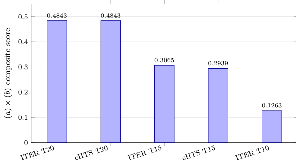
Figure 3: F-funnel (a) \times (b) composite scores for the five design points of Table 3. The two T=20 keV points (ITER-class and compact-HTS) tie at 0.4843; the score falls with operating temperature as the reactivity ceiling ( a ) dominates. Data: verify atoms f_reactivity_coverage / f_margin_coverage / f_funnel_composite (■ SUPPORTED-NUMERICAL, |\Delta| = 0 , PR #1020).
