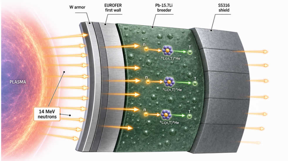
Figure 8: Conceptual DEMO breeding-blanket cross-section for pipeline stage ⑨ (gate f): 14.06 MeV DT neutrons stream from the plasma side (left) through the W armor and EUROFER first wall into the Pb-15.7Li breeder, where the {}^6\text{Li}(n, \alpha)\text{T} reaction breeds tritium, with the SS316 shield outboard. The to-scale radial build and the OpenMC TBR = 1.3222 result are in Fig. 9 and Table 14. Image generated via fal.ai gpt-image-2 (prompt: figures/_prompts/fig_blanket_concept.txt ; commons @D g44) — illustrative, not a verified data figure.
