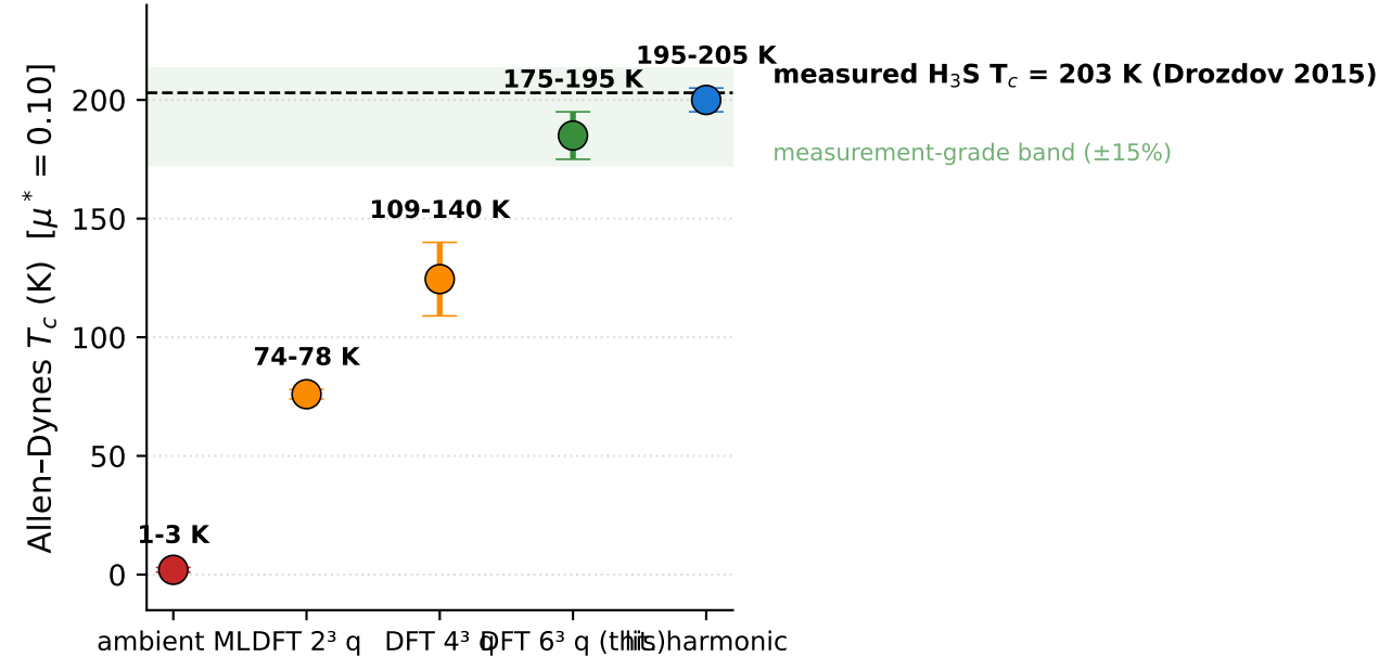
H 3 S Allen-Dynes T c convergence vs phonon q-grid
