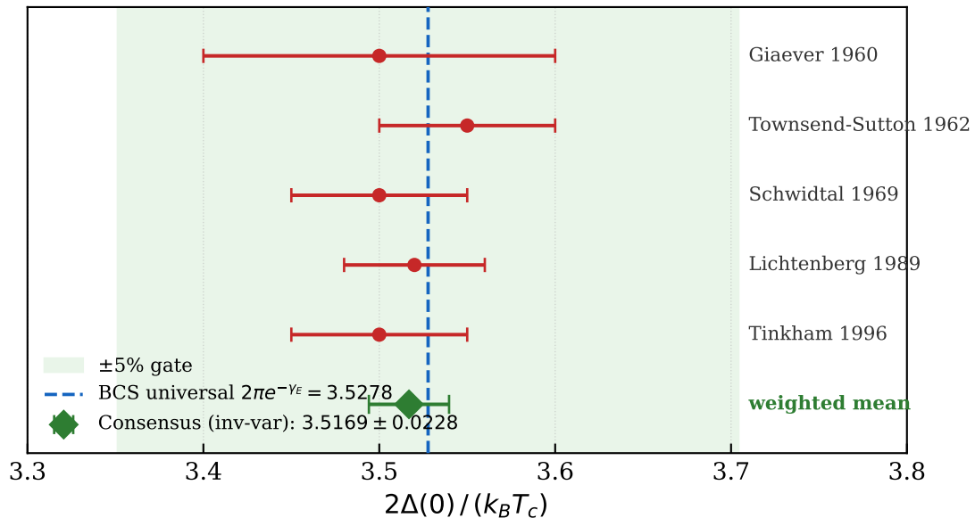
Nb tunneling consensus vs BCS prediction (rel.\,err.\, = 0.309%)
