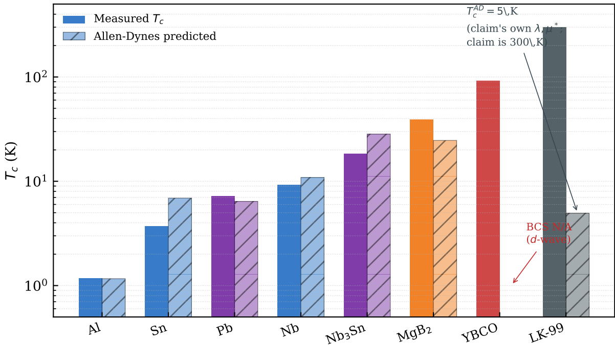
BCS-class T_c prediction vs measurement across SC families
