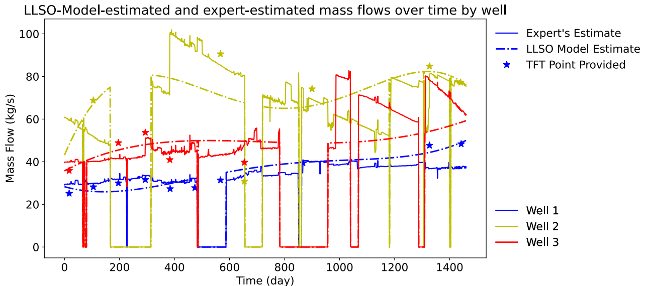
Figure 4.2: Mass flows predicted by LLSO model for real data, for k = 5 with optimal regularisation parameter values. This somewhat follows the trend of the TFT points, similarly to the expert's estimate. However, it does differ in places, especially for Well 2 which varies the most sharply. It does best with Well 1 because Well 1 provides the most TFT points.
