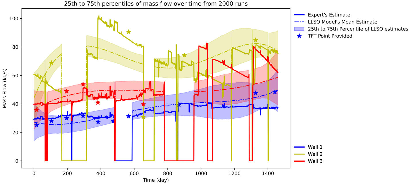
Figure 4.3: 25th to 75th percentiles of mass flows predicted by LLSO model for real data, for k = 5 and optimal parameter values. These percentiles graphically show the uncertainty of the prediction for each well and timepoint. There is more uncertainty when TFT points are not provided nearby, and there is more uncertainty at the edged of the time-domain.
