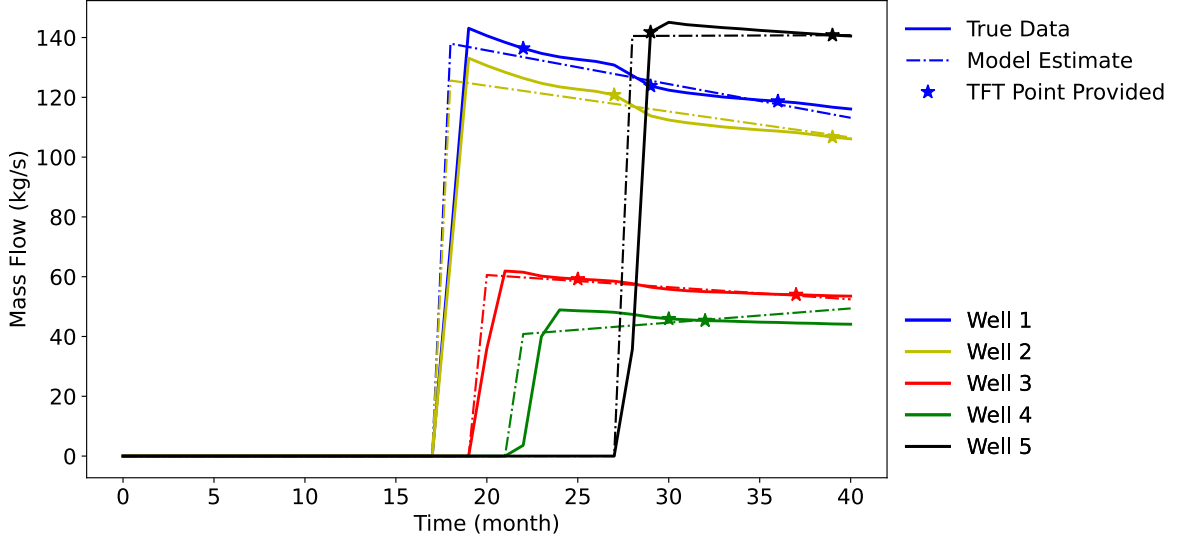
Figure 2.2: Mass flows predicted by linear LFO Model against true mass flows. This improves on the constant LFO model by allowing the model to represent the real behaviour more accurately, and decreases the RMSE to 10.34.
