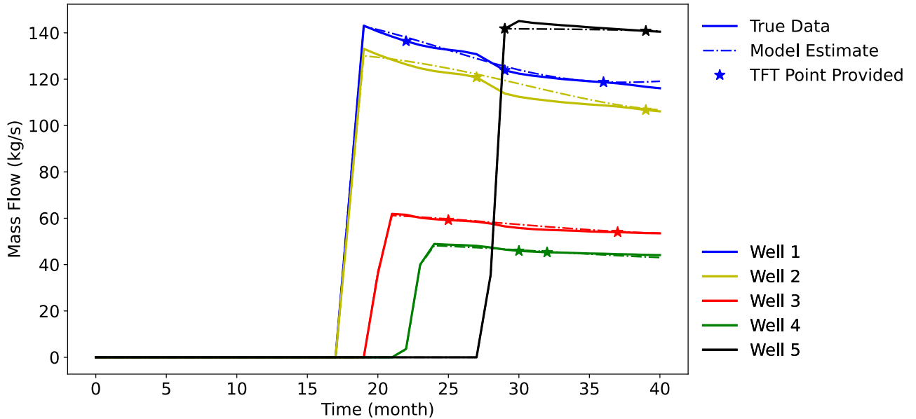
Figure 4.1: Mass flows predicted by LLSO model for simulated data, for k = 5 and optimal parameter values found using particle swarm optimisation. The RMSE for this prediction is 1.139.
