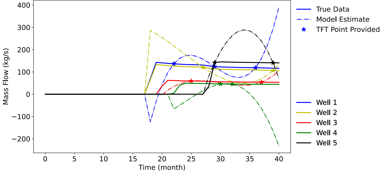
Figure 2.4: Mass flows predicted by AHOP LFO model for k=3 (cubic) against true mass flows. This prediction is clearly a poor one, as it is overfitting to the provided data. It is nearly perfectly matching each TFT point, but is modelling unrealistic behaviour between these points. The RMSE of this model is 13.24, which is significantly worse than previous models.
