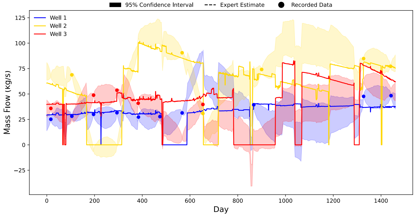
Figure 4.4: 95% confidence intervals of Michael's GPR Model for real data. This shows a highly variable prediction because each sample is enforced to go exactly through each TFT point. Adapted from [34]
