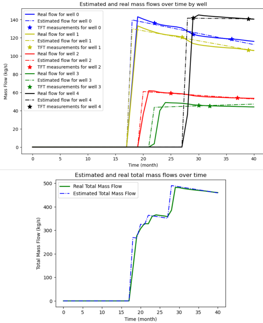
Figure 3.2: Mass flows predicted by linear model against real results for individual wells and total flows.
