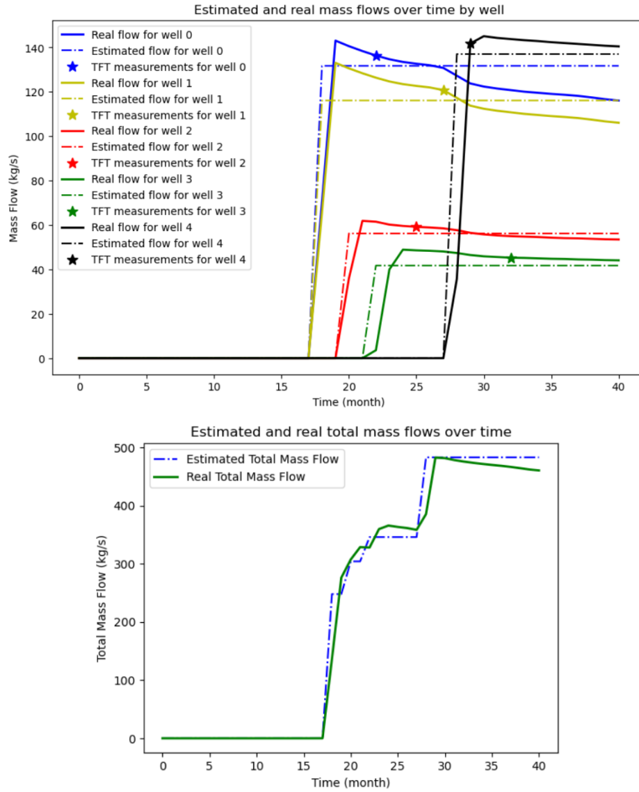
Figure 3.1: Mass flows predicted by initial model against real results for individual wells and total flows.
