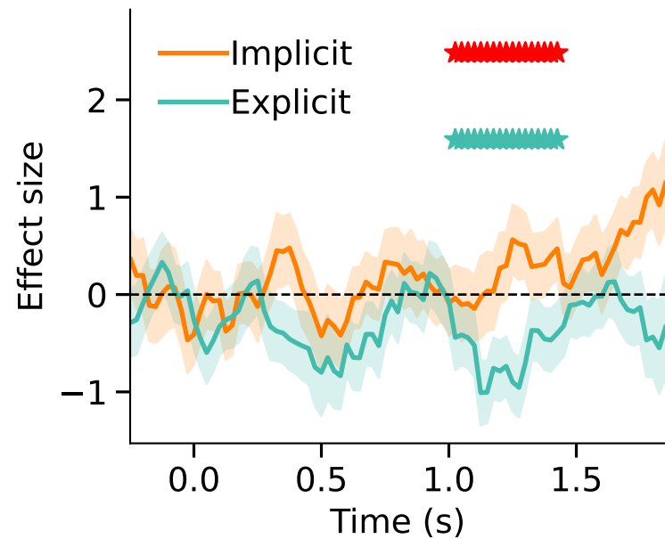
VIS: next trial reach RT
