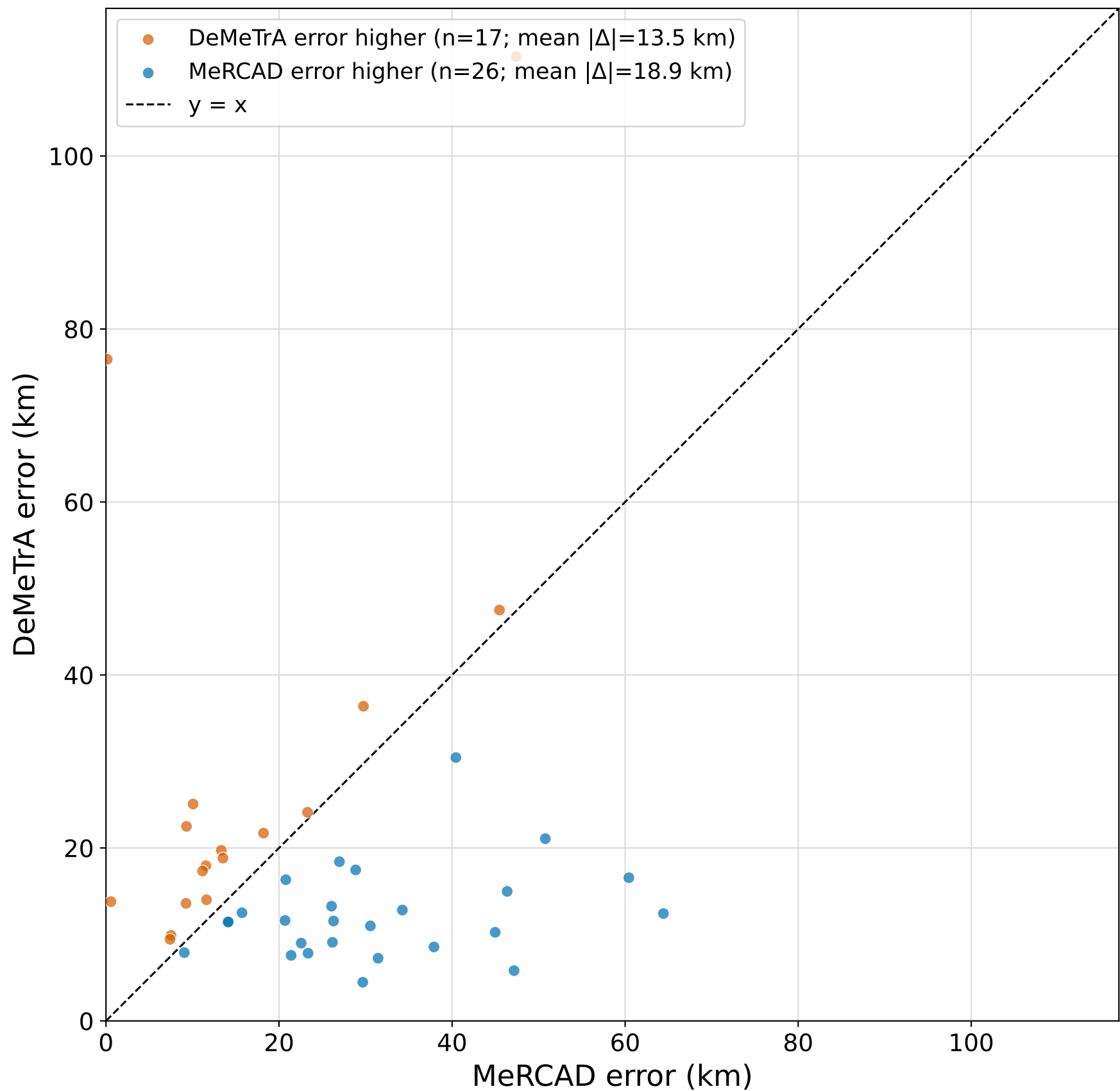
Paired comparison of DeMeTrA and MeRCAD cyclone-centre errors
